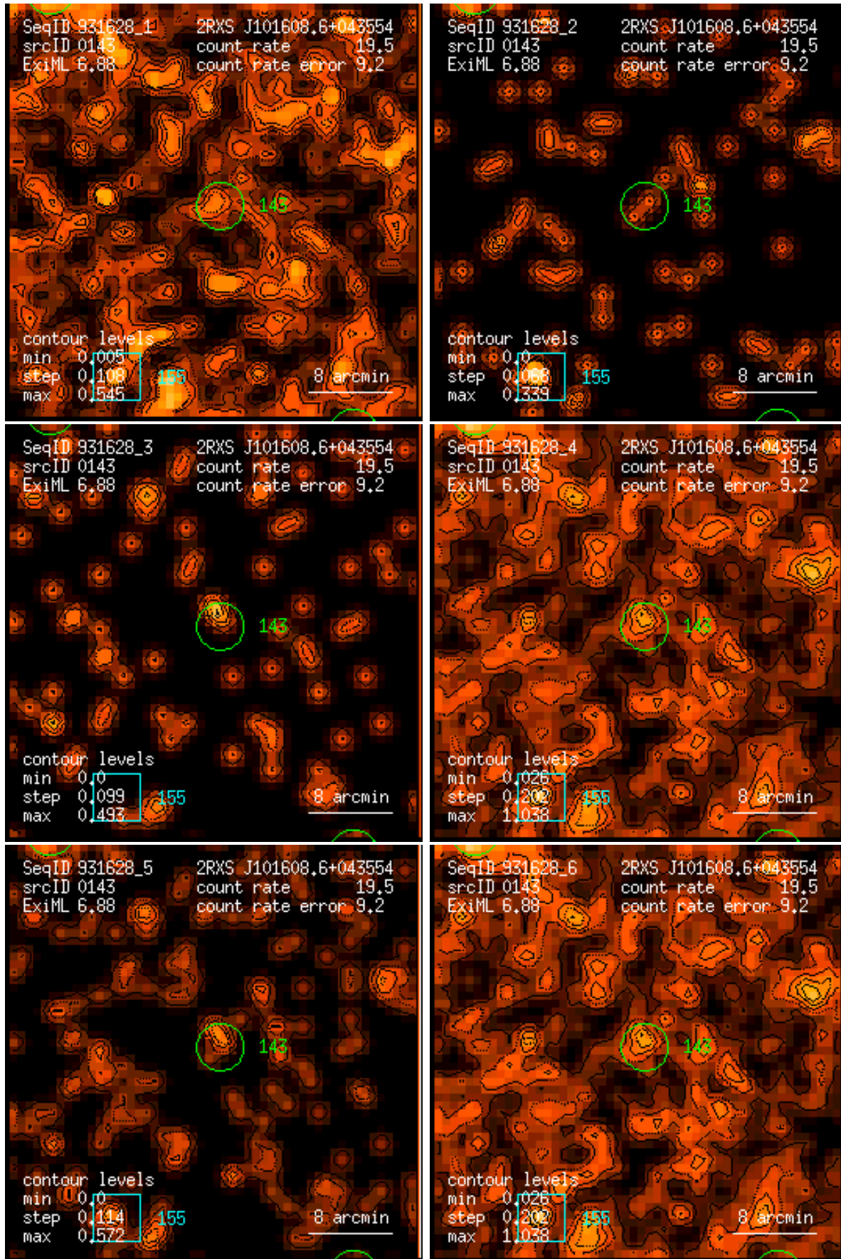
Figure 143: RASS 931628: detection 0143: band rate images, Gaussian filter: (1) PSPC channels 11 – 41, (2) 52 – 90, (3) 91 – 201, (4) 11 – 235, (5) 52 – 201, (6) 11 – 201. Broad band rates in counts/ks. Band rate contour levels in counts/ks/arcmin 2 .
