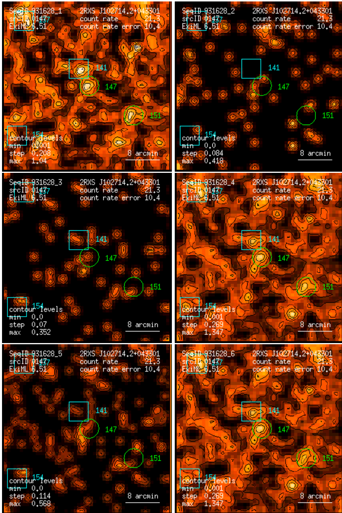
Figure 147: RASS 931628: detection 0147: band rate images, Gaussian filter: (1) PSPC channels 11 – 41, (2) 52 – 90, (3) 91 – 201, (4) 11 – 235, (5) 52 – 201, (6) 11 – 201. Broad band rates in counts/ks. Band rate contour levels in counts/ks/arcmin 2 .
