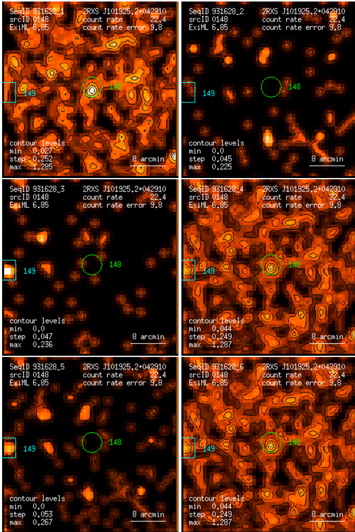
Figure 148: RASS 931628: detection 0148: band rate images, Gaussian filter: (1) PSPC channels 11 – 41, (2) 52 – 90, (3) 91 – 201, (4) 11 – 235, (5) 52 – 201, (6) 11 – 201. Broad band rates in counts/ks. Band rate contour levels in counts/ks/arcmin 2 .
