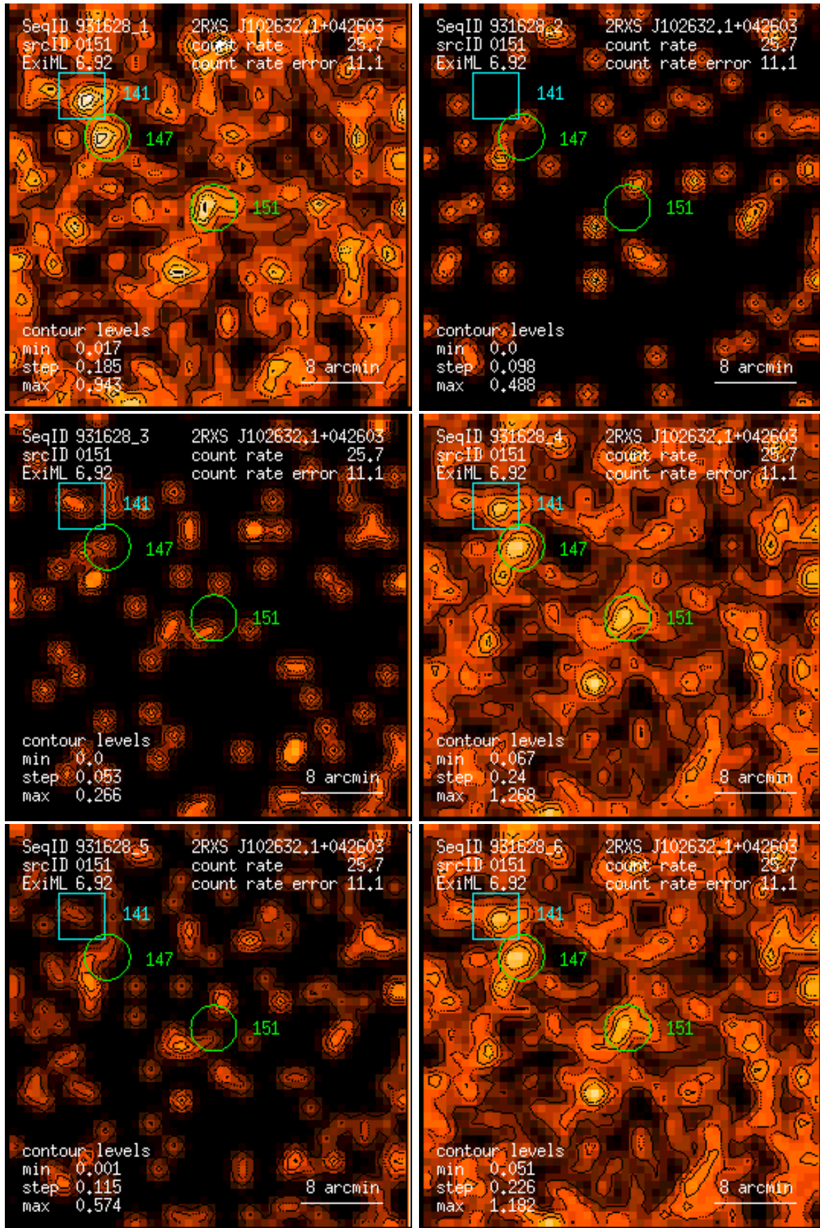
Figure 151: RASS 931628: detection 0151: band rate images, Gaussian filter: (1) PSPC channels 11 – 41, (2) 52 – 90, (3) 91 – 201, (4) 11 – 235, (5) 52 – 201, (6) 11 – 201. Broad band rates in counts/ks. Band rate contour levels in counts/ks/arcmin 2 .
