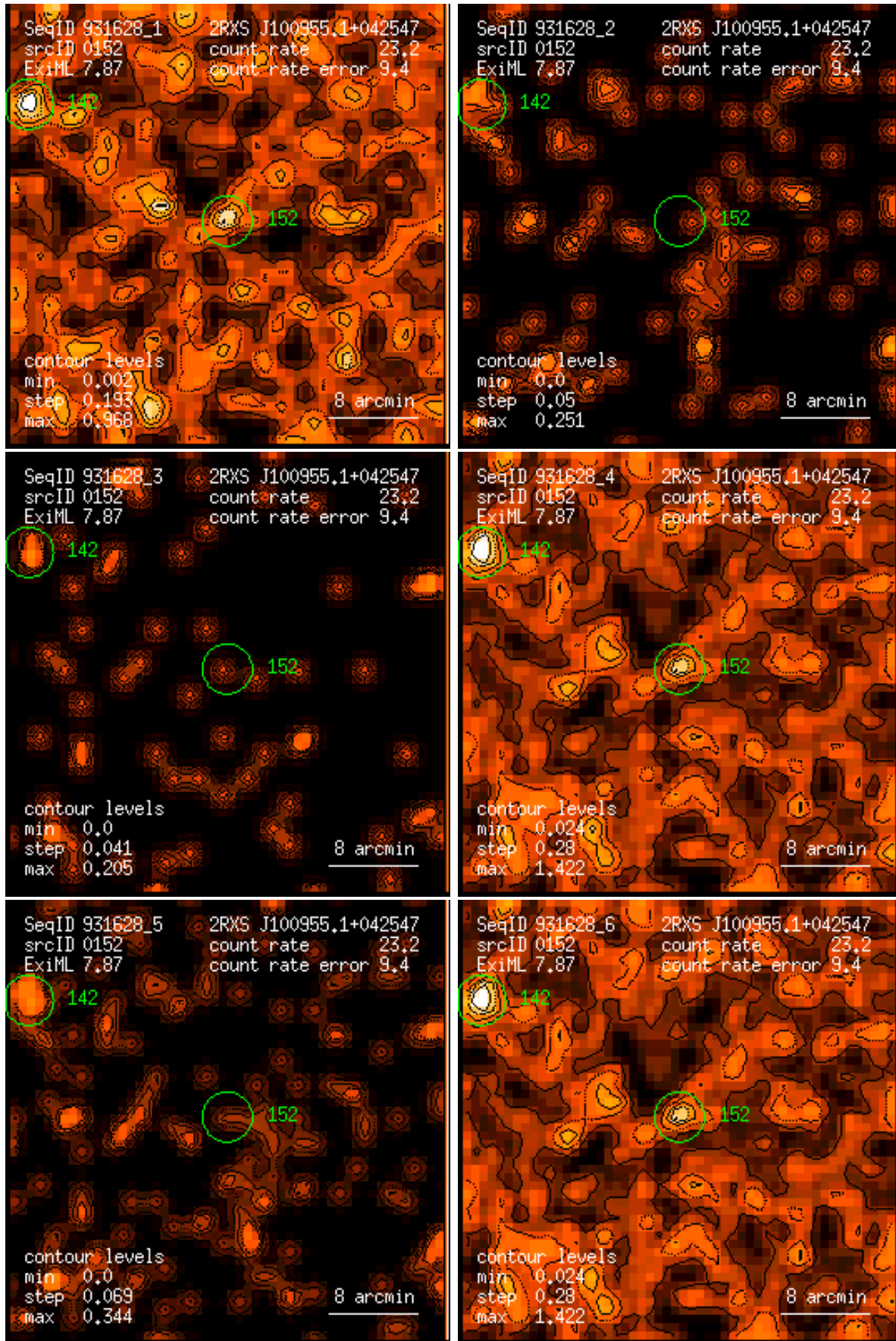
Figure 152: RASS 931628: detection 0152: band rate images, Gaussian filter: (1) PSPC channels 11 – 41, (2) 52 – 90, (3) 91 – 201, (4) 11 – 235, (5) 52 – 201, (6) 11 – 201. Broad band rates in counts/ks. Band rate contour levels in counts/ks/arcmin 2 .
