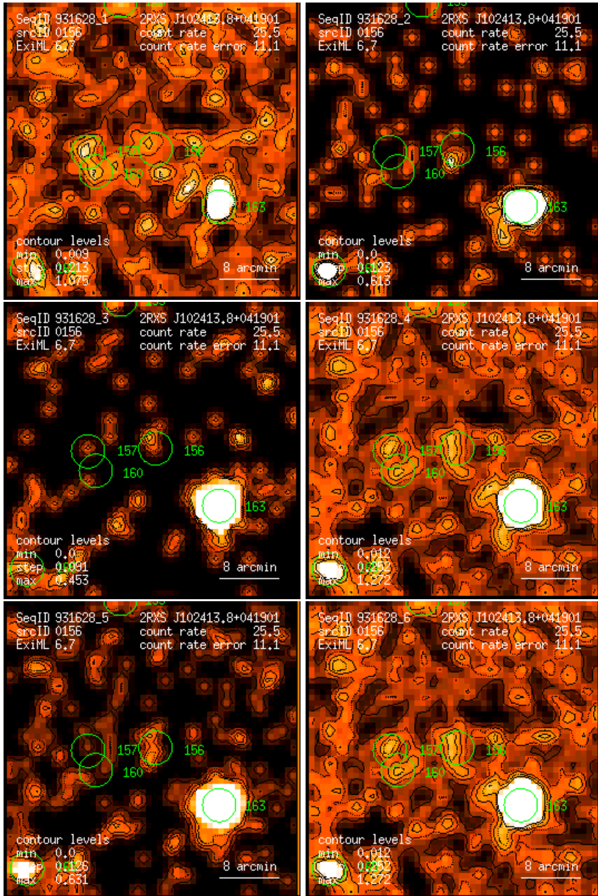
Figure 156: RASS 931628: detection 0156: band rate images, Gaussian filter: (1) PSPC channels 11 – 41, (2) 52 – 90, (3) 91 – 201, (4) 11 – 235, (5) 52 – 201, (6) 11 – 201. Broad band rates in counts/ks. Band rate contour levels in counts/ks/arcmin 2 .
