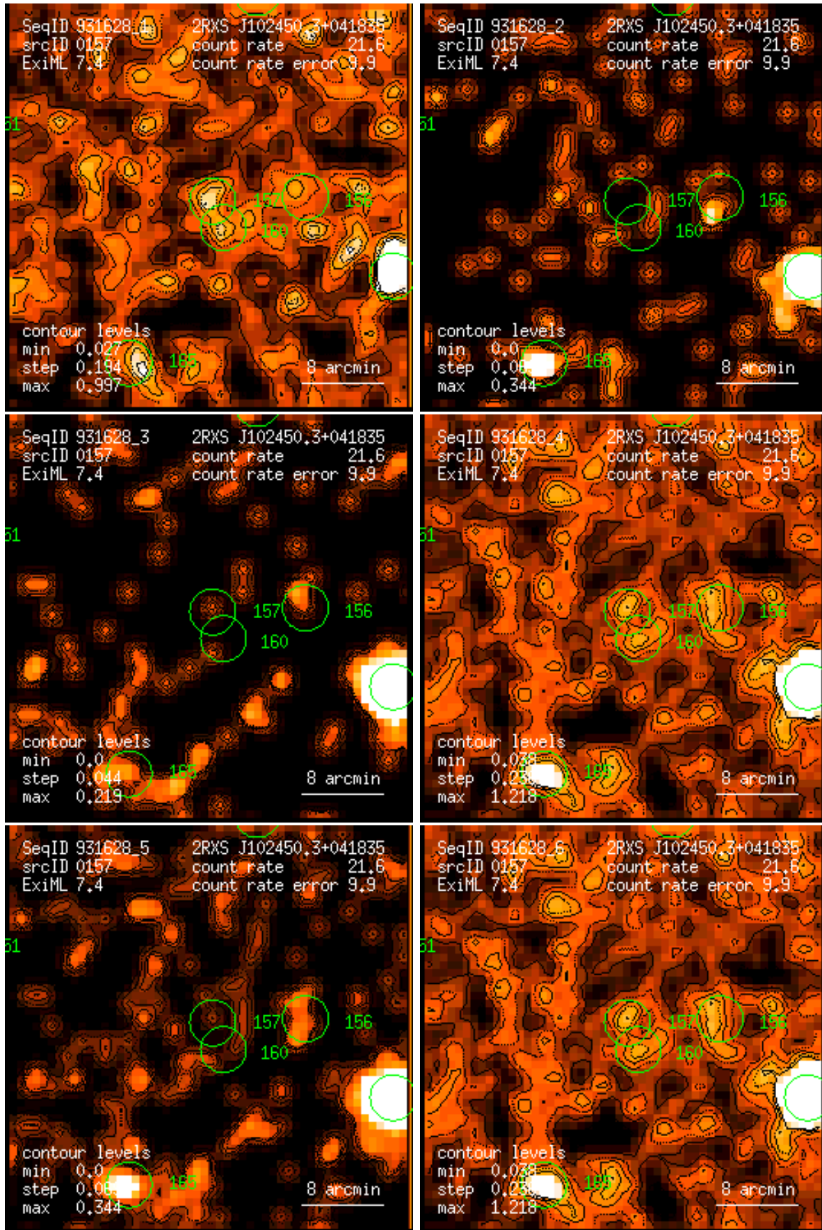
Figure 157: RASS 931628: detection 0157: band rate images, Gaussian filter: (1) PSPC channels 11 – 41, (2) 52 – 90, (3) 91 – 201, (4) 11 – 235, (5) 52 – 201, (6) 11 – 201. Broad band rates in counts/ks. Band rate contour levels in counts/ks/arcmin 2 .
