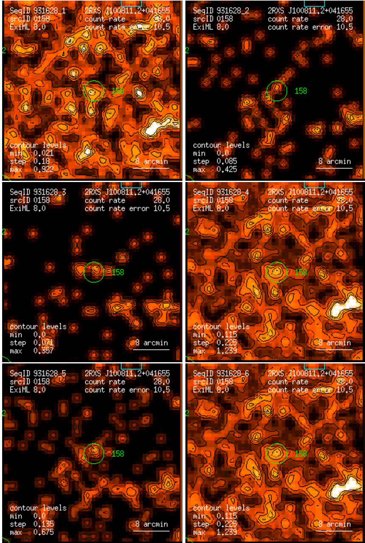
Figure 158: RASS 931628: detection 0158: band rate images, Gaussian filter: (1) PSPC channels 11 – 41, (2) 52 – 90, (3) 91 – 201, (4) 11 – 235, (5) 52 – 201, (6) 11 – 201. Broad band rates in counts/ks. Band rate contour levels in counts/ks/arcmin 2 .
