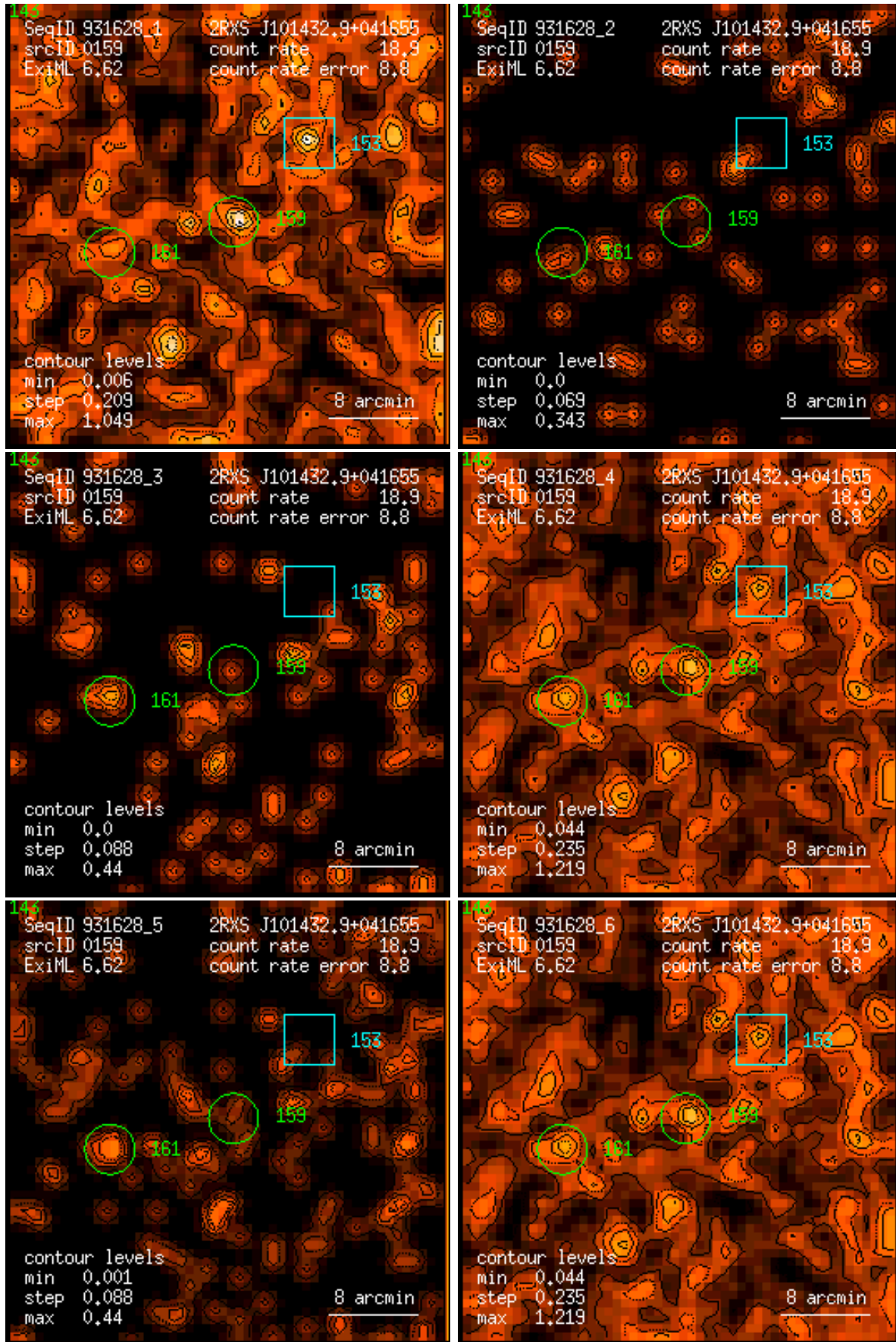
Figure 159: RASS 931628: detection 0159: band rate images, Gaussian filter: (1) PSPC channels 11 – 41, (2) 52 – 90, (3) 91 – 201, (4) 11 – 235, (5) 52 – 201, (6) 11 – 201. Broad band rates in counts/ks. Band rate contour levels in counts/ks/arcmin 2 .
