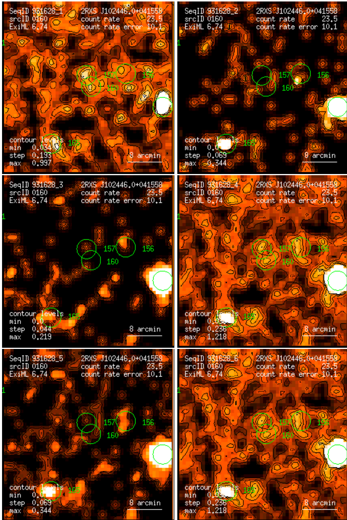
Figure 160: RASS 931628: detection 0160: band rate images, Gaussian filter: (1) PSPC channels 11 – 41, (2) 52 – 90, (3) 91 – 201, (4) 11 – 235, (5) 52 – 201, (6) 11 – 201. Broad band rates in counts/ks. Band rate contour levels in counts/ks/arcmin 2 .
