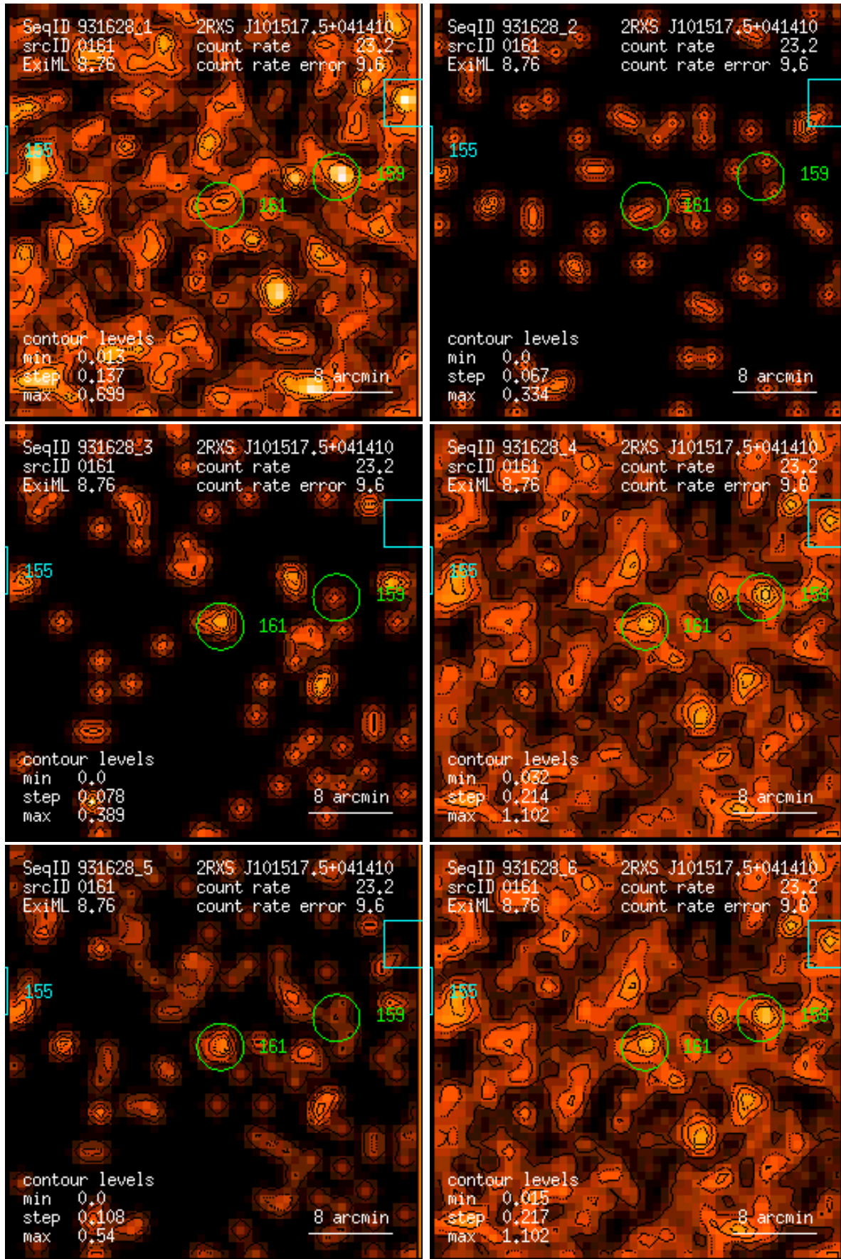
Figure 161: RASS 931628: detection 0161: band rate images, Gaussian filter: (1) PSPC channels 11 – 41, (2) 52 – 90, (3) 91 – 201, (4) 11 – 235, (5) 52 – 201, (6) 11 – 201. Broad band rates in counts/ks. Band rate contour levels in counts/ks/arcmin 2 .
