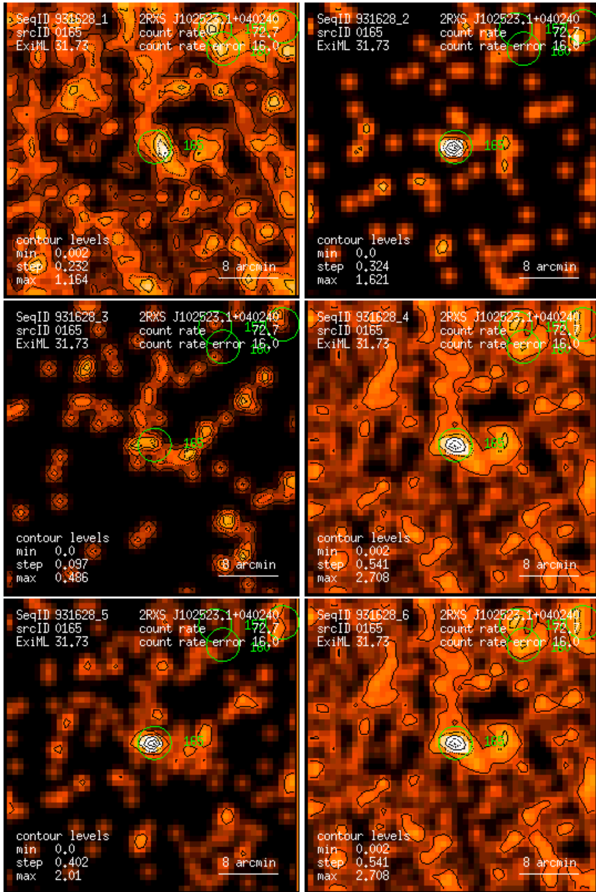
Figure 165: RASS 931628: detection 0165: band rate images, Gaussian filter: (1) PSPC channels 11 – 41, (2) 52 – 90, (3) 91 – 201, (4) 11 – 235, (5) 52 – 201, (6) 11 – 201. Broad band rates in counts/ks. Band rate contour levels in counts/ks/arcmin 2 .
