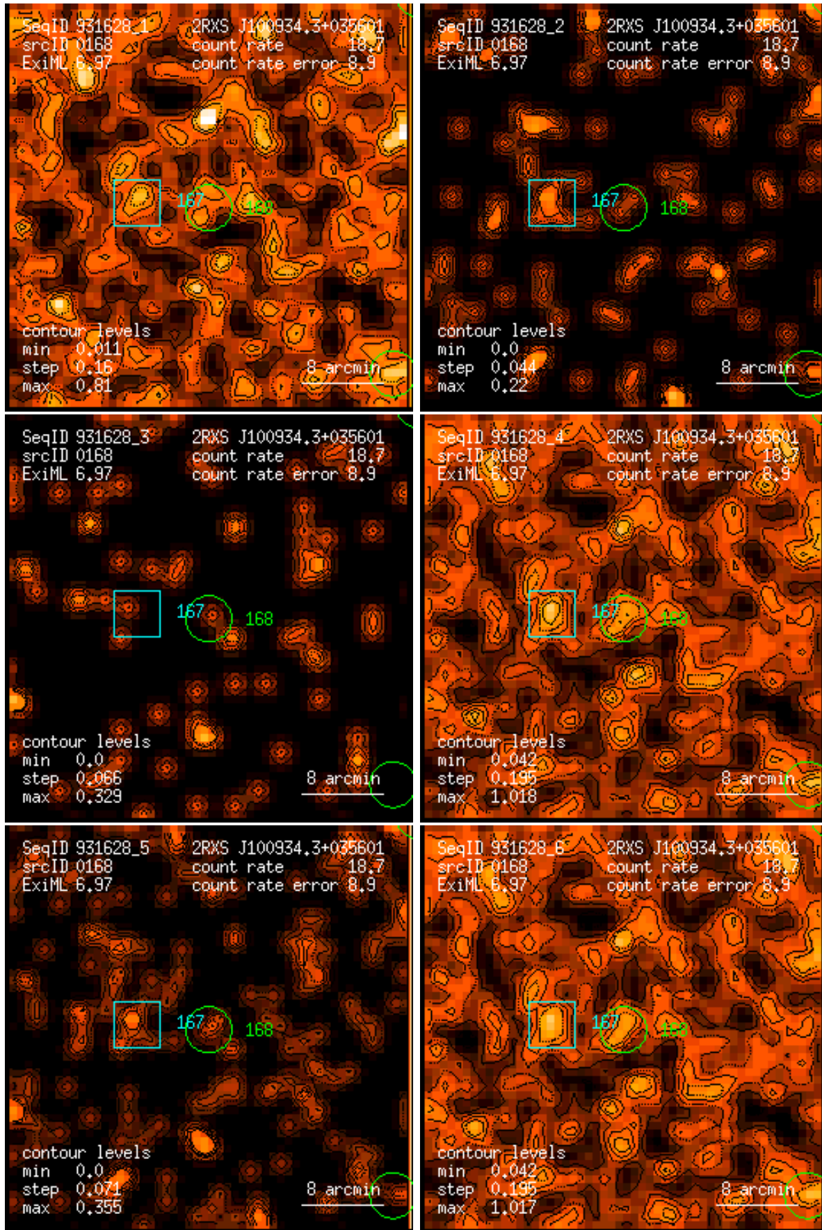
Figure 168: RASS 931628: detection 0168: band rate images, Gaussian filter: (1) PSPC channels 11 – 41, (2) 52 – 90, (3) 91 – 201, (4) 11 – 235, (5) 52 – 201, (6) 11 – 201. Broad band rates in counts/ks. Band rate contour levels in counts/ks/arcmin 2 .
