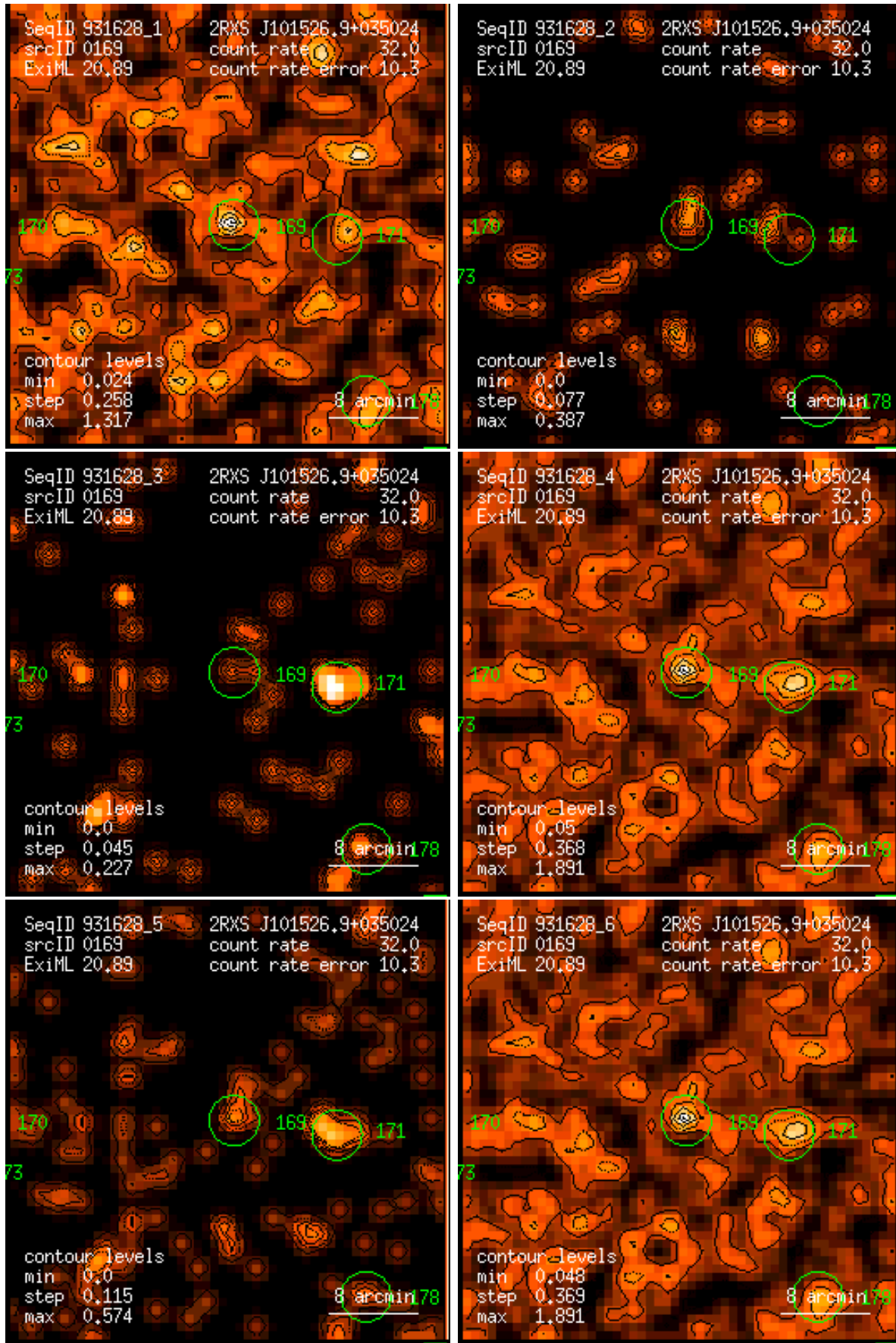
Figure 169: RASS 931628: detection 0169: band rate images, Gaussian filter: (1) PSPC channels 11 – 41, (2) 52 – 90, (3) 91 – 201, (4) 11 – 235, (5) 52 – 201, (6) 11 – 201. Broad band rates in counts/ks. Band rate contour levels in counts/ks/arcmin 2 .
