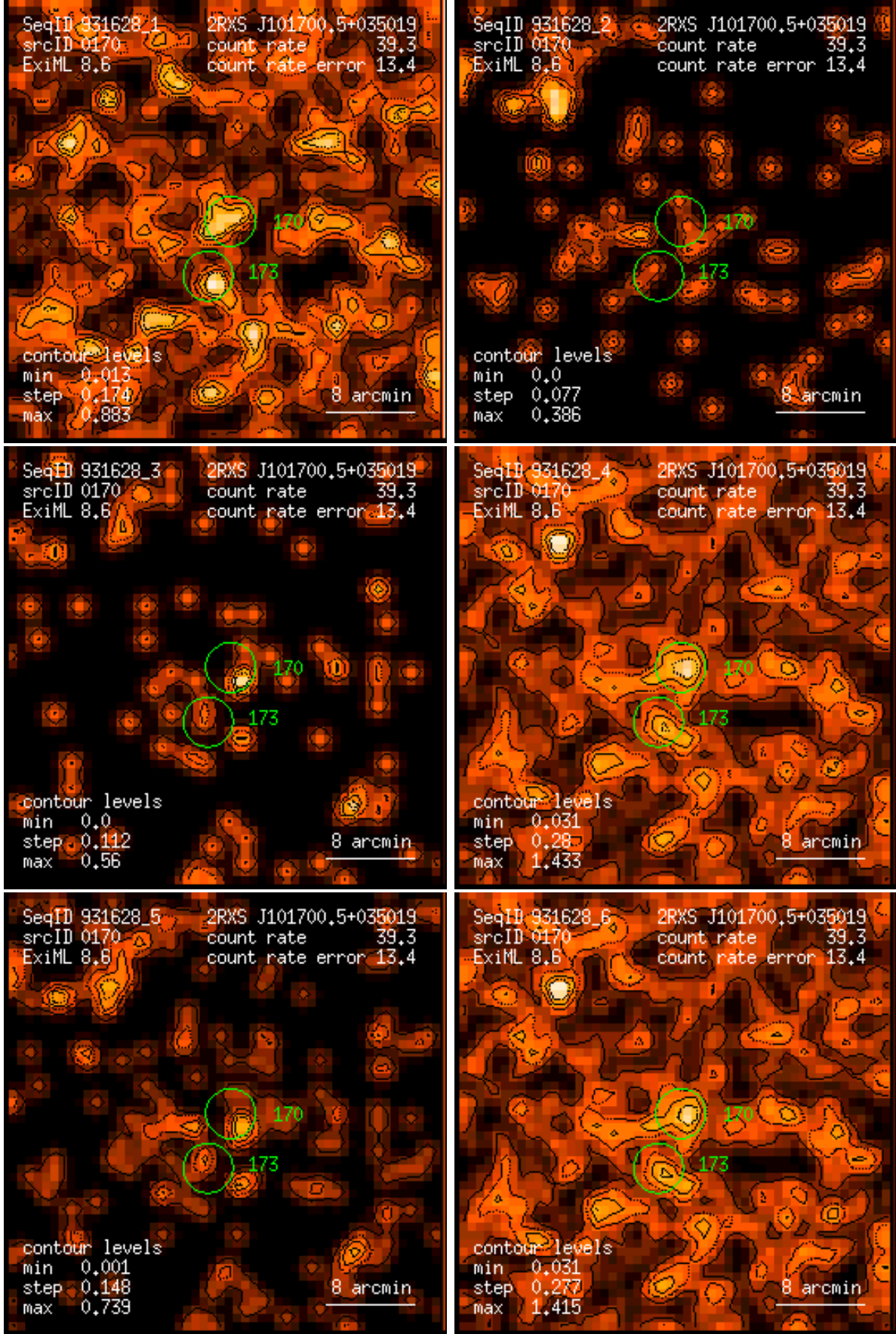
Figure 170: RASS 931628: detection 0170: band rate images, Gaussian filter: (1) PSPC channels 11 – 41, (2) 52 – 90, (3) 91 – 201, (4) 11 – 235, (5) 52 – 201, (6) 11 – 201. Broad band rates in counts/ks. Band rate contour levels in counts/ks/arcmin 2 .
