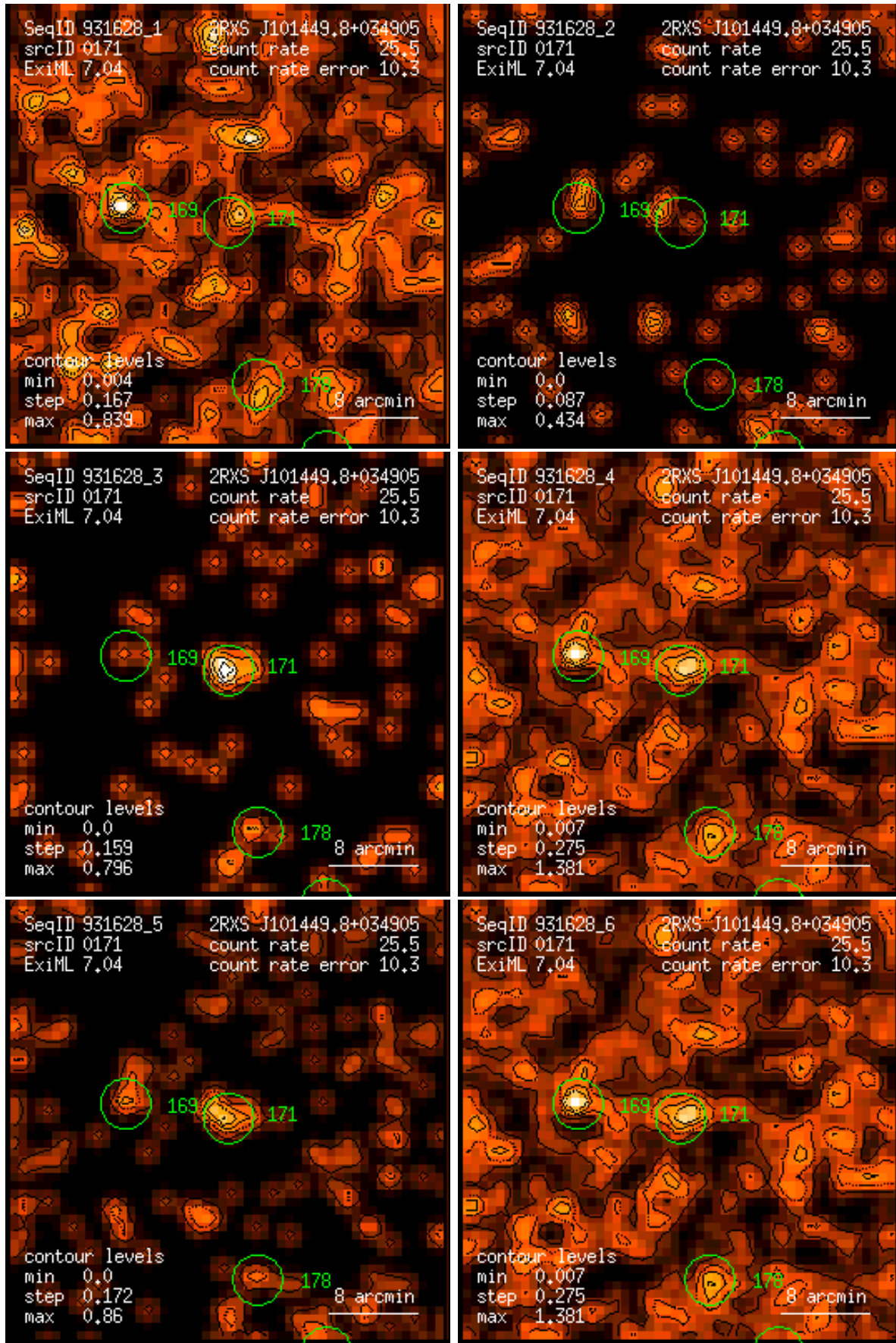
Figure 171: RASS 931628: detection 0171: band rate images, Gaussian filter: (1) PSPC channels 11 – 41, (2) 52 – 90, (3) 91 – 201, (4) 11 – 235, (5) 52 – 201, (6) 11 – 201. Broad band rates in counts/ks. Band rate contour levels in counts/ks/arcmin 2 .
