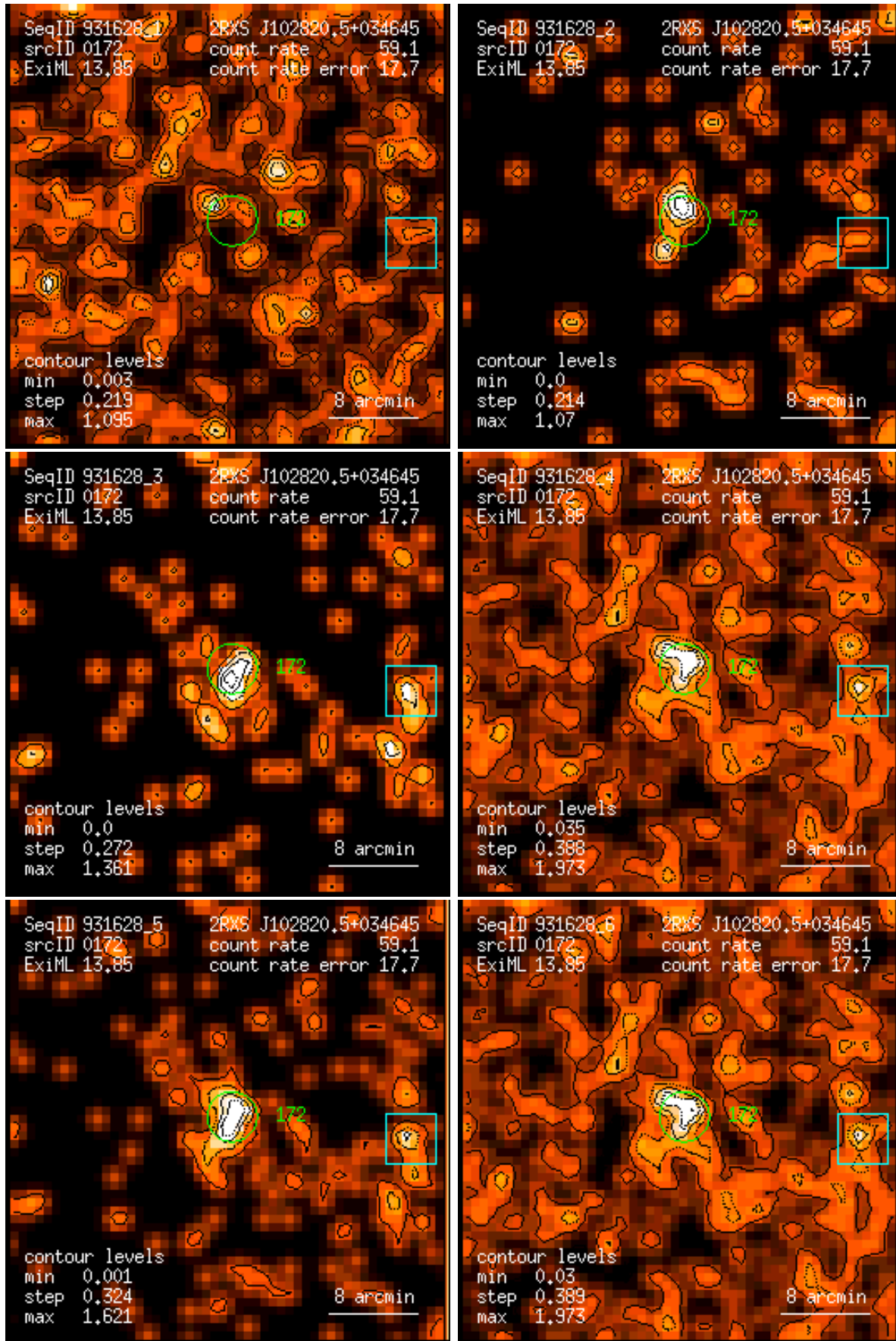
Figure 172: RASS 931628: detection 0172: band rate images, Gaussian filter: (1) PSPC channels 11 – 41, (2) 52 – 90, (3) 91 – 201, (4) 11 – 235, (5) 52 – 201, (6) 11 – 201. Broad band rates in counts/ks. Band rate contour levels in counts/ks/arcmin 2 .
