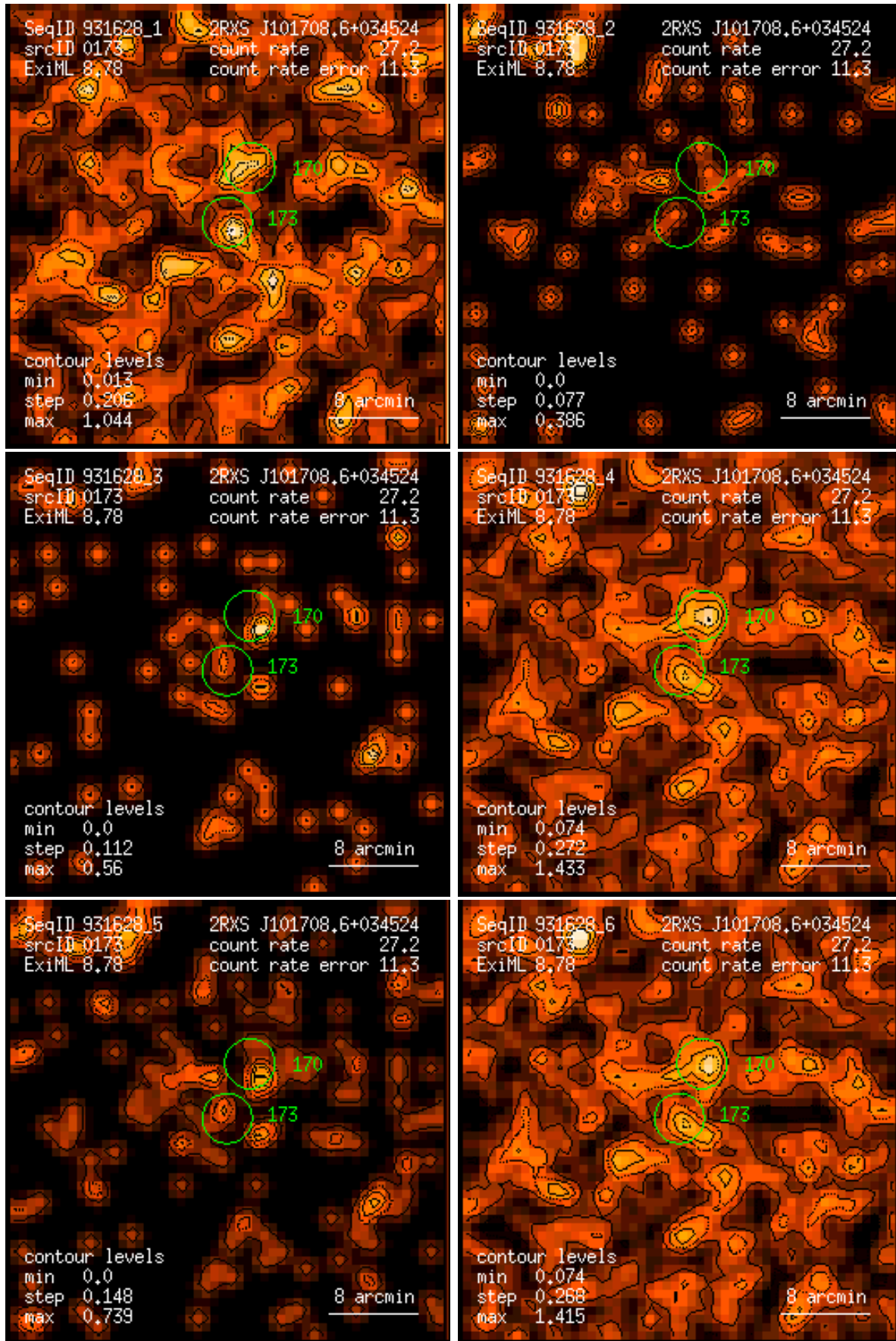
Figure 173: RASS 931628: detection 0173: band rate images, Gaussian filter: (1) PSPC channels 11 – 41, (2) 52 – 90, (3) 91 – 201, (4) 11 – 235, (5) 52 – 201, (6) 11 – 201. Broad band rates in counts/ks. Band rate contour levels in counts/ks/arcmin 2 .
