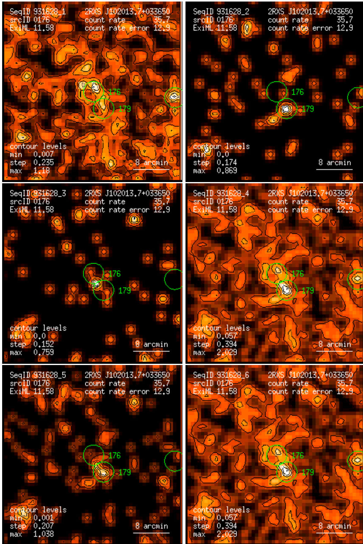
Figure 176: RASS 931628: detection 0176: band rate images, Gaussian filter: (1) PSPC channels 11 – 41, (2) 52 – 90, (3) 91 – 201, (4) 11 – 235, (5) 52 – 201, (6) 11 – 201. Broad band rates in counts/ks. Band rate contour levels in counts/ks/arcmin 2 .
