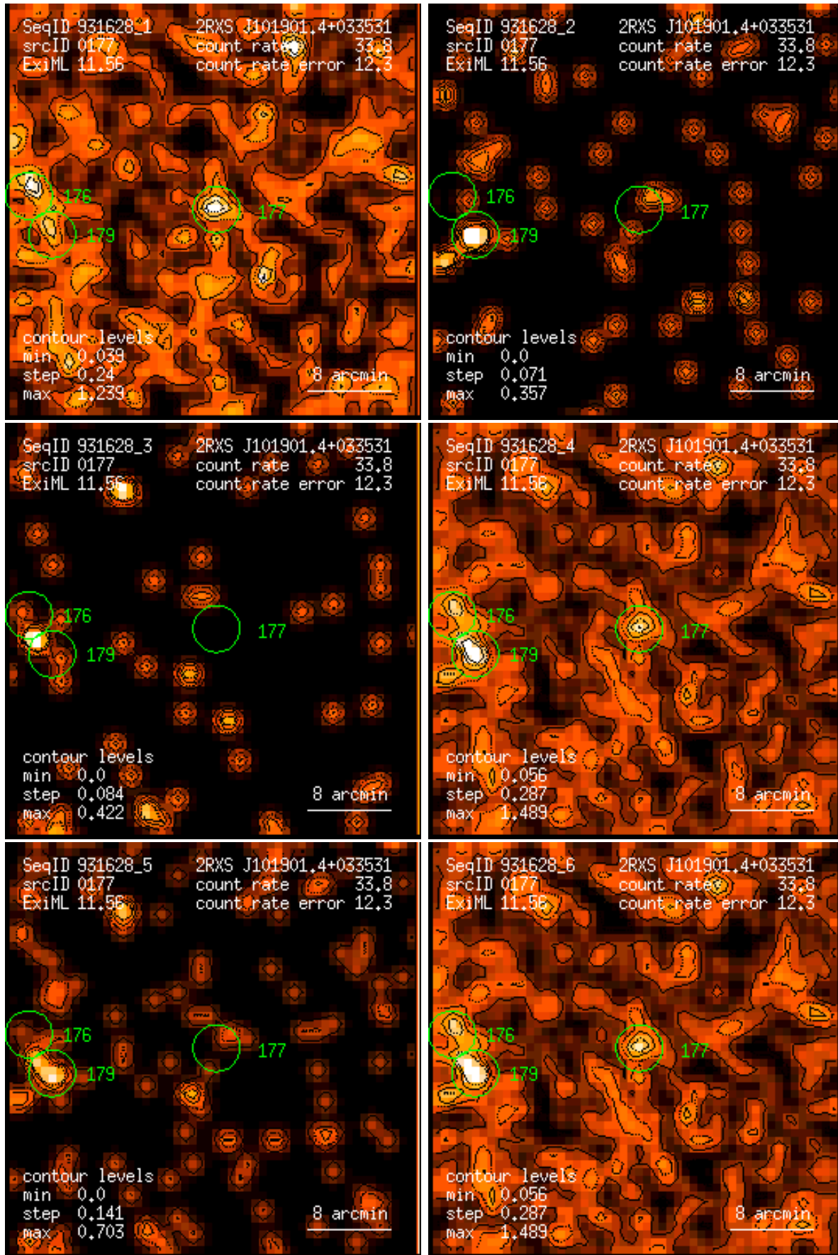
Figure 177: RASS 931628: detection 0177: band rate images, Gaussian filter: (1) PSPC channels 11 – 41, (2) 52 – 90, (3) 91 – 201, (4) 11 – 235, (5) 52 – 201, (6) 11 – 201. Broad band rates in counts/ks. Band rate contour levels in counts/ks/arcmin 2 .
