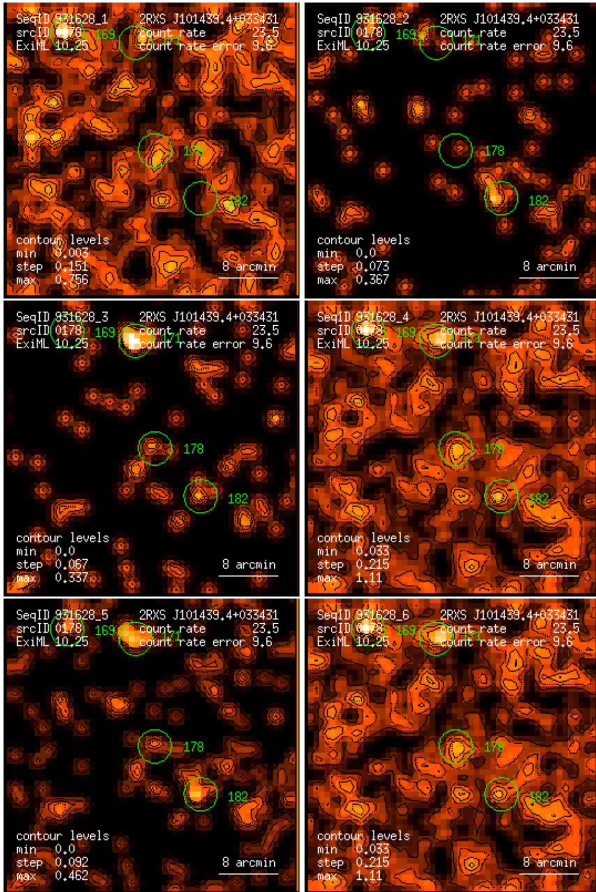
Figure 178: RASS 931628: detection 0178: band rate images, Gaussian filter: (1) PSPC channels 11 – 41, (2) 52 – 90, (3) 91 – 201, (4) 11 – 235, (5) 52 – 201, (6) 11 – 201. Broad band rates in counts/ks. Band rate contour levels in counts/ks/arcmin 2 .
