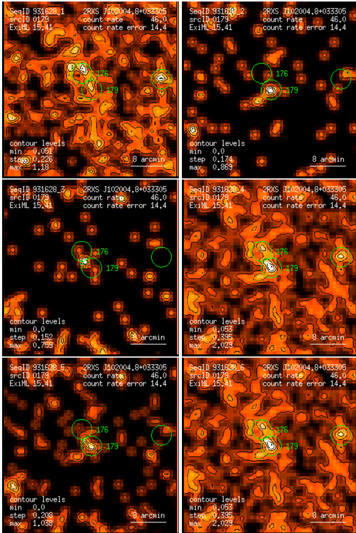
Figure 179: RASS 931628: detection 0179: band rate images, Gaussian filter: (1) PSPC channels 11 – 41, (2) 52 – 90, (3) 91 – 201, (4) 11 – 235, (5) 52 – 201, (6) 11 – 201. Broad band rates in counts/ks. Band rate contour levels in counts/ks/arcmin 2 .
