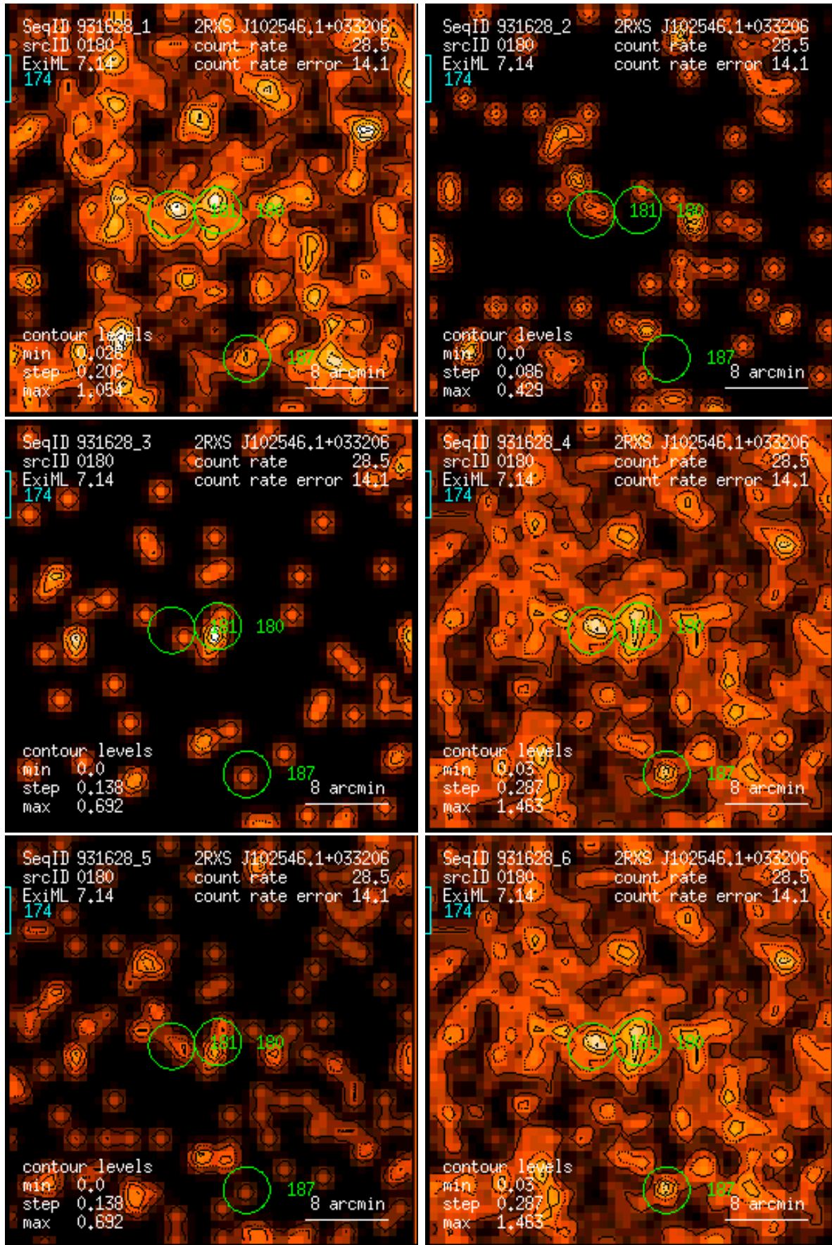
Figure 180: RASS 931628: detection 0180: band rate images, Gaussian filter: (1) PSPC channels 11 – 41, (2) 52 – 90, (3) 91 – 201, (4) 11 – 235, (5) 52 – 201, (6) 11 – 201. Broad band rates in counts/ks. Band rate contour levels in counts/ks/arcmin 2 .
