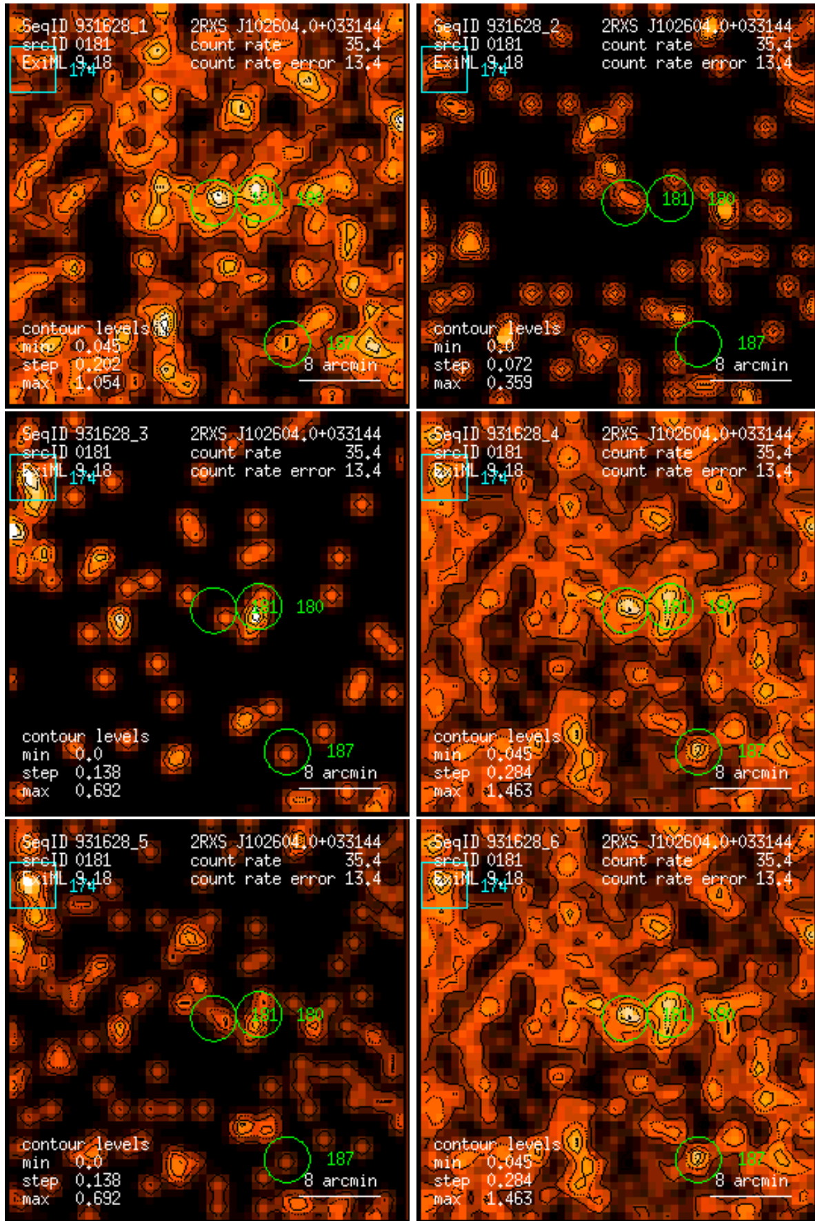
Figure 181: RASS 931628: detection 0181: band rate images, Gaussian filter: (1) PSPC channels 11 – 41, (2) 52 – 90, (3) 91 – 201, (4) 11 – 235, (5) 52 – 201, (6) 11 – 201. Broad band rates in counts/ks. Band rate contour levels in counts/ks/arcmin 2 .
