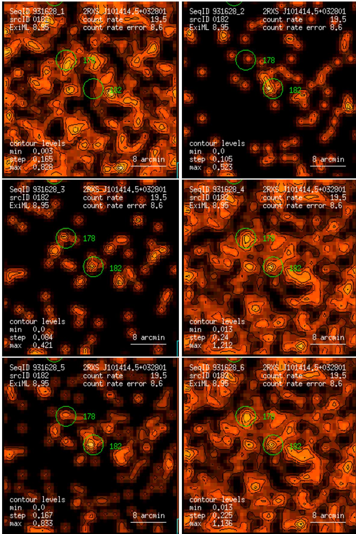
Figure 182: RASS 931628: detection 0182: band rate images, Gaussian filter: (1) PSPC channels 11 – 41, (2) 52 – 90, (3) 91 – 201, (4) 11 – 235, (5) 52 – 201, (6) 11 – 201. Broad band rates in counts/ks. Band rate contour levels in counts/ks/arcmin 2 .
