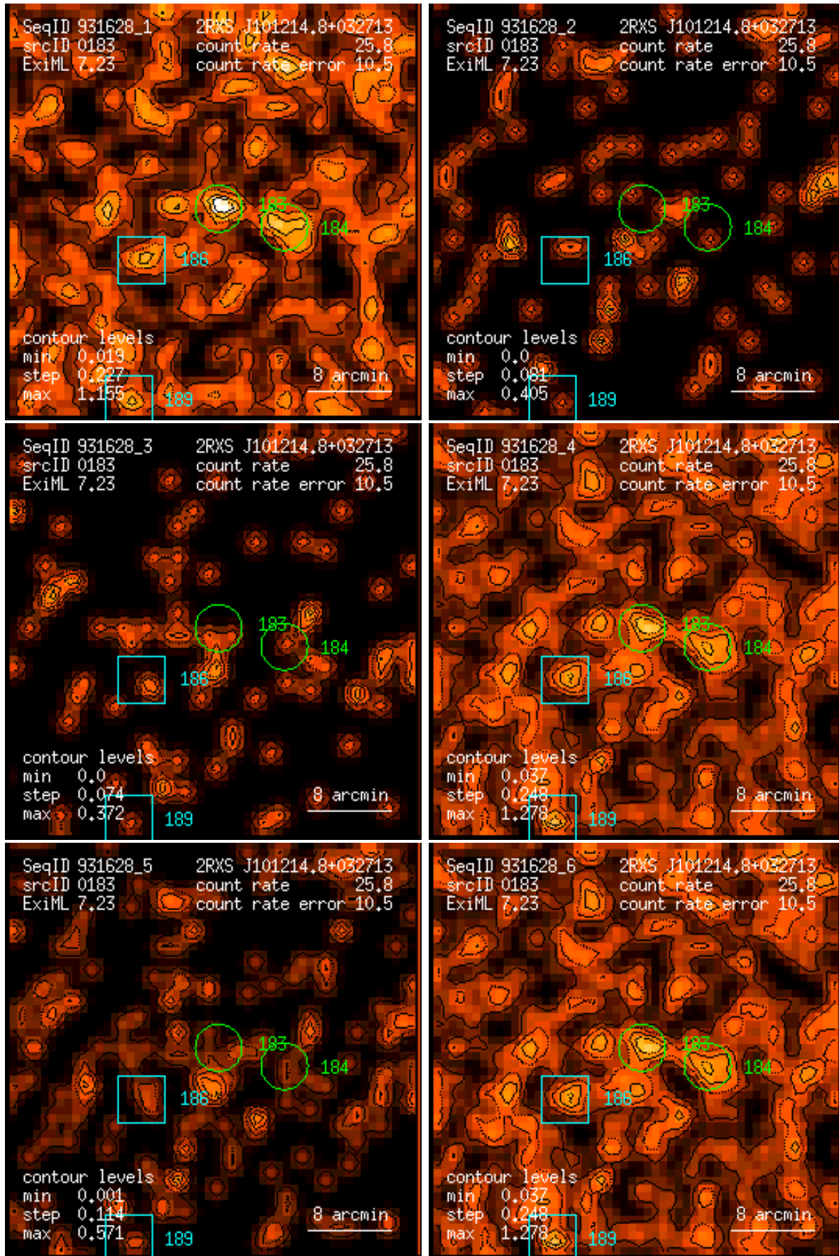
Figure 183: RASS 931628: detection 0183: band rate images, Gaussian filter: (1) PSPC channels 11 – 41, (2) 52 – 90, (3) 91 – 201, (4) 11 – 235, (5) 52 – 201, (6) 11 – 201. Broad band rates in counts/ks. Band rate contour levels in counts/ks/arcmin 2 .
