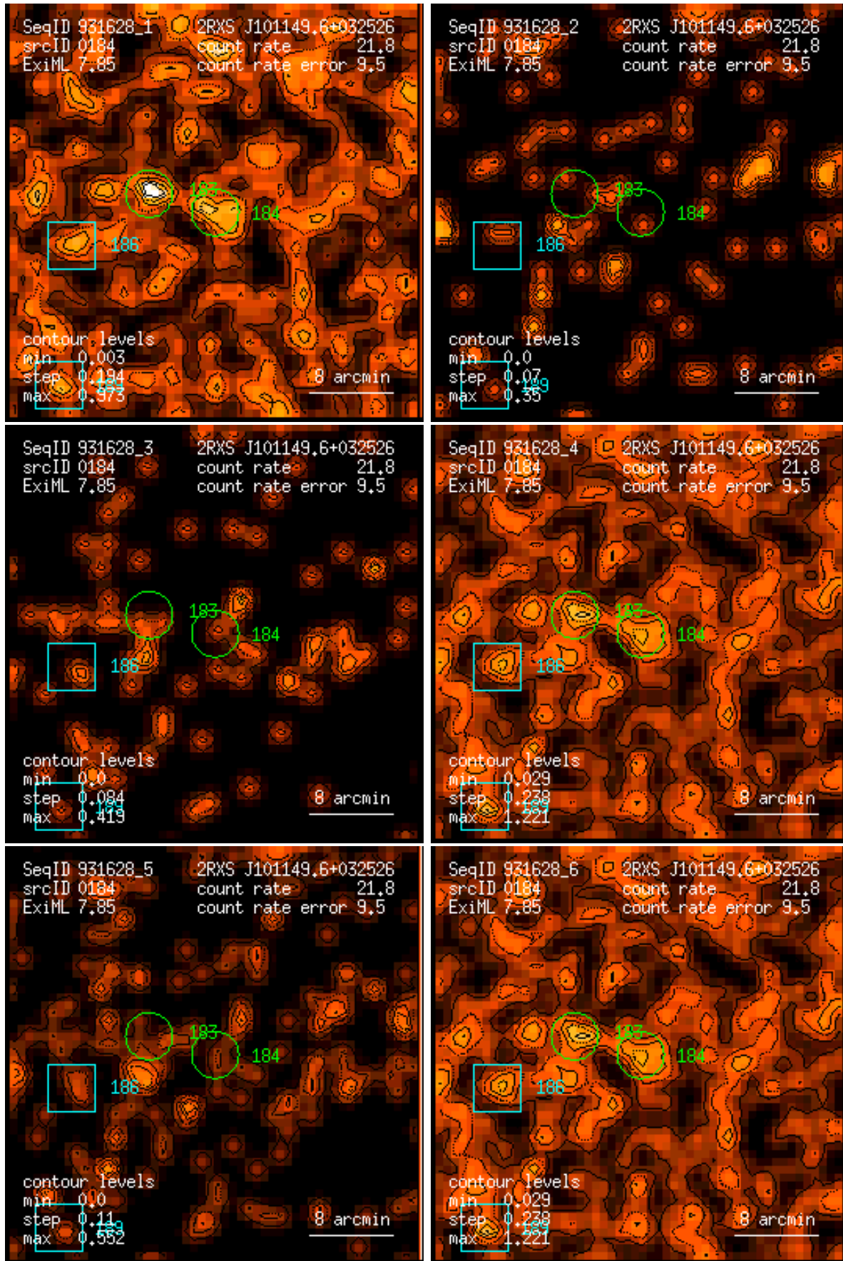
Figure 184: RASS 931628: detection 0184: band rate images, Gaussian filter: (1) PSPC channels 11 – 41, (2) 52 – 90, (3) 91 – 201, (4) 11 – 235, (5) 52 – 201, (6) 11 – 201. Broad band rates in counts/ks. Band rate contour levels in counts/ks/arcmin 2 .
