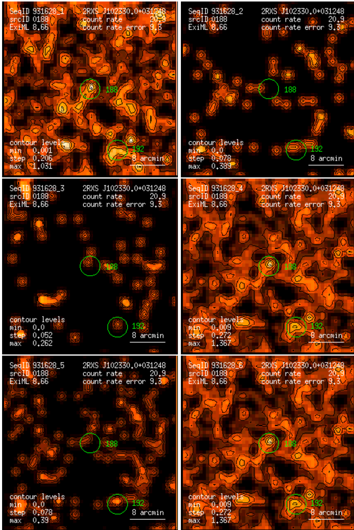
Figure 188: RASS 931628: detection 0188: band rate images, Gaussian filter: (1) PSPC channels 11 – 41, (2) 52 – 90, (3) 91 – 201, (4) 11 – 235, (5) 52 – 201, (6) 11 – 201. Broad band rates in counts/ks. Band rate contour levels in counts/ks/arcmin 2 .
