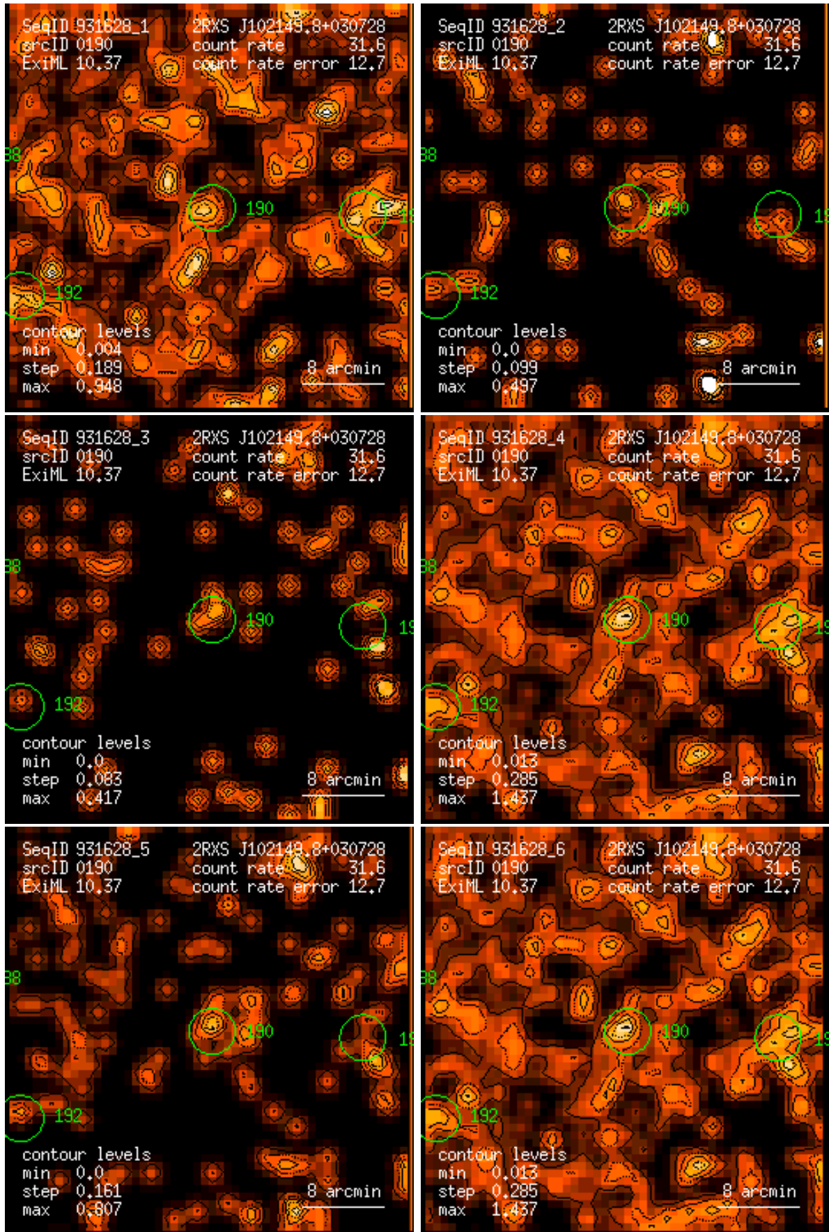
Figure 190: RASS 931628: detection 0190: band rate images, Gaussian filter: (1) PSPC channels 11 – 41, (2) 52 – 90, (3) 91 – 201, (4) 11 – 235, (5) 52 – 201, (6) 11 – 201. Broad band rates in counts/ks. Band rate contour levels in counts/ks/arcmin 2 .
