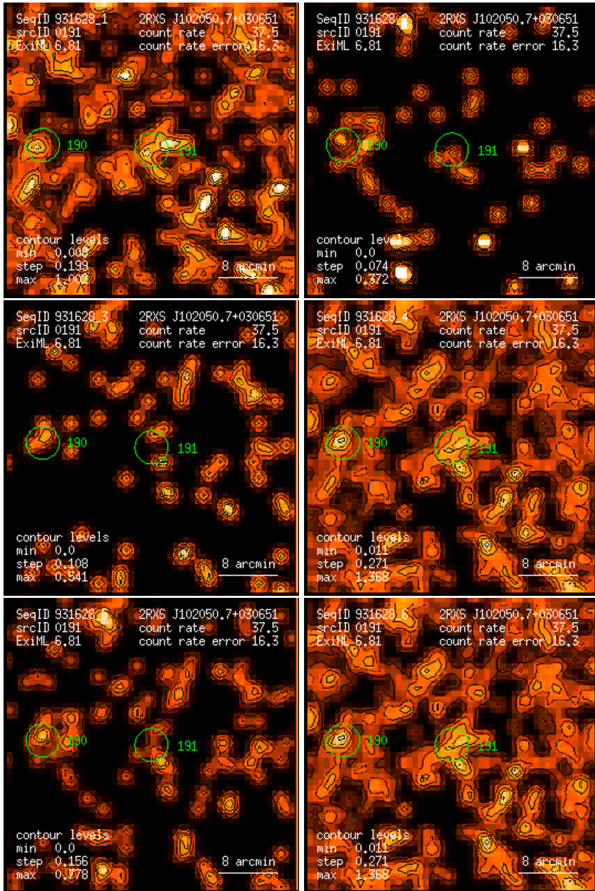
Figure 191: RASS 931628: detection 0191: band rate images, Gaussian filter: (1) PSPC channels 11 – 41, (2) 52 – 90, (3) 91 – 201, (4) 11 – 235, (5) 52 – 201, (6) 11 – 201. Broad band rates in counts/ks. Band rate contour levels in counts/ks/arcmin 2 .
