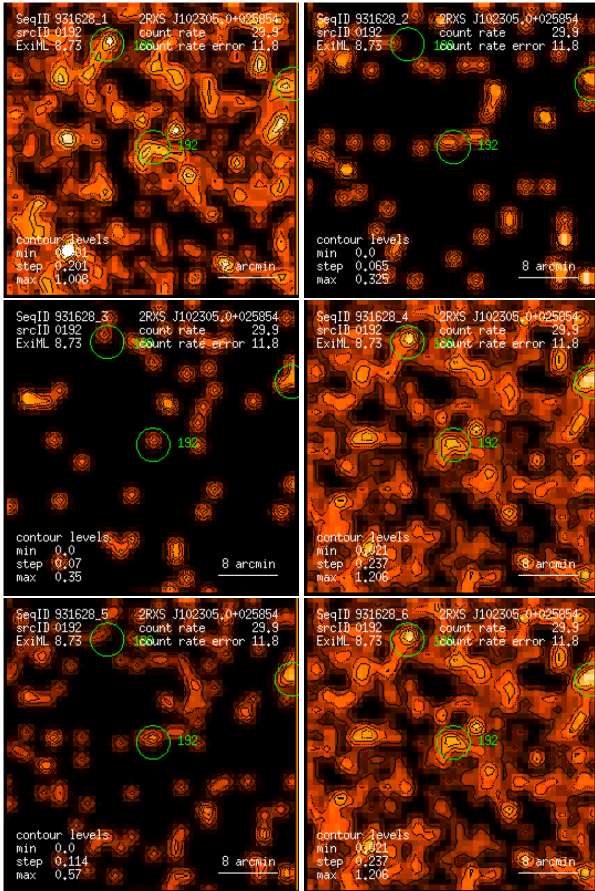
Figure 192: RASS 931628: detection 0192: band rate images, Gaussian filter: (1) PSPC channels 11 – 41, (2) 52 – 90, (3) 91 – 201, (4) 11 – 235, (5) 52 – 201, (6) 11 – 201. Broad band rates in counts/ks. Band rate contour levels in counts/ks/arcmin 2 .
