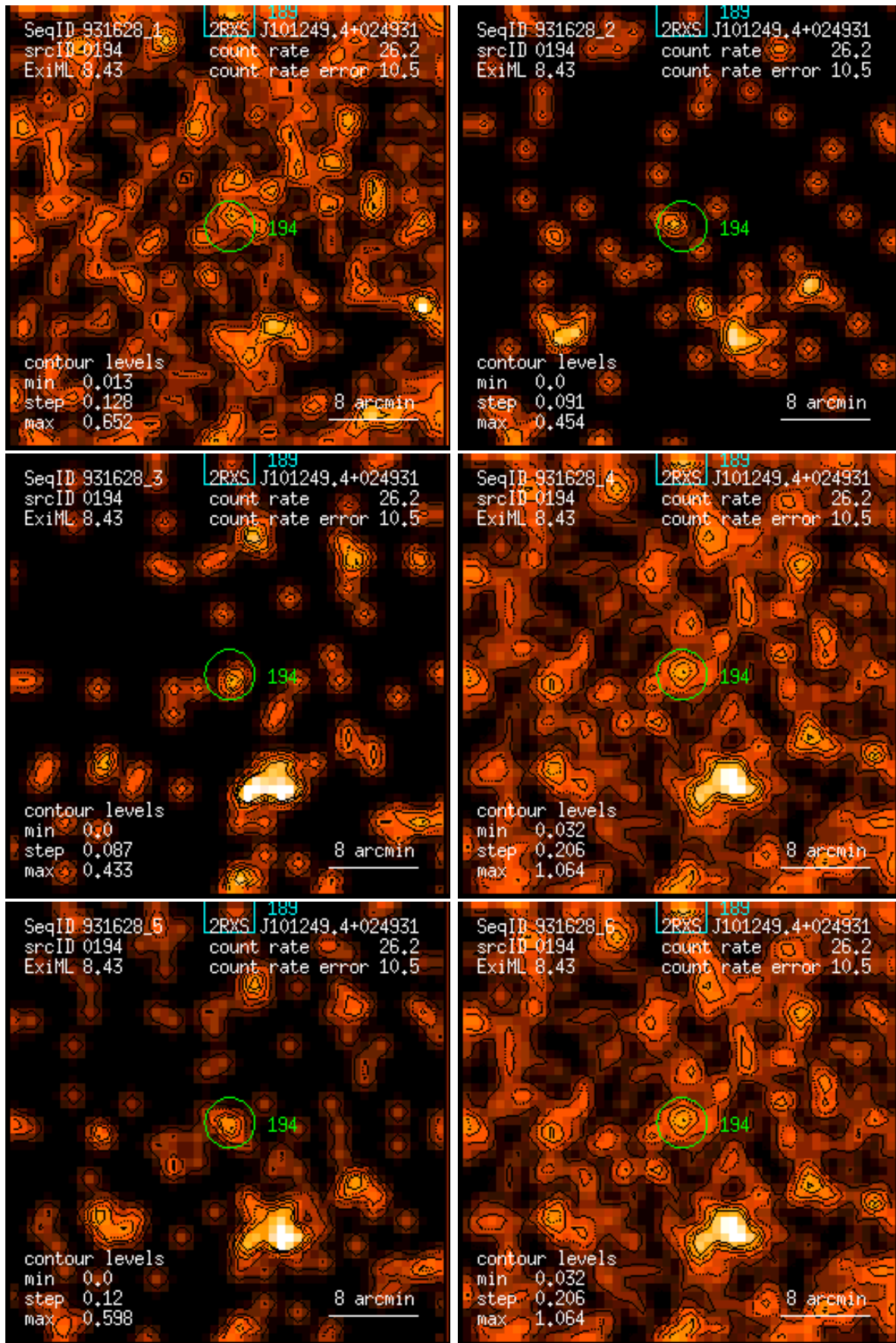
Figure 194: RASS 931628: detection 0194: band rate images, Gaussian filter: (1) PSPC channels 11 – 41, (2) 52 – 90, (3) 91 – 201, (4) 11 – 235, (5) 52 – 201, (6) 11 – 201. Broad band rates in counts/ks. Band rate contour levels in counts/ks/arcmin 2 .
