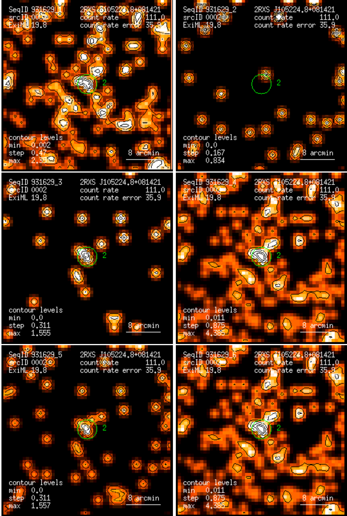
Figure 2: RASS 931629: detection 0002: band rate images, Gaussian filter: (1) PSPC channels 11 – 41, (2) 52 – 90, (3) 91 – 201, (4) 11 – 235, (5) 52 – 201, (6) 11 – 201. Broad band rates in counts/ks. Band rate contour levels in counts/ks/arcmin 2 .
