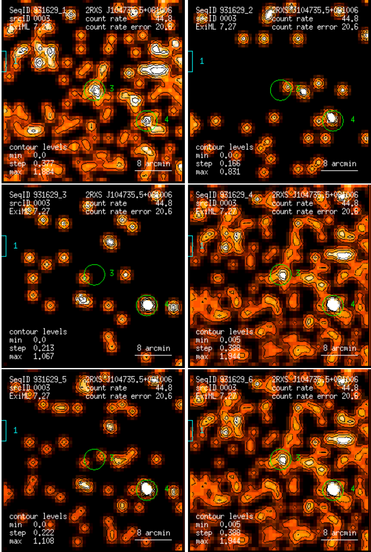
Figure 3: RASS 931629: detection 0003: band rate images, Gaussian filter: (1) PSPC channels 11 – 41, (2) 52 – 90, (3) 91 – 201, (4) 11 – 235, (5) 52 – 201, (6) 11 – 201. Broad band rates in counts/ks. Band rate contour levels in counts/ks/arcmin 2 .
