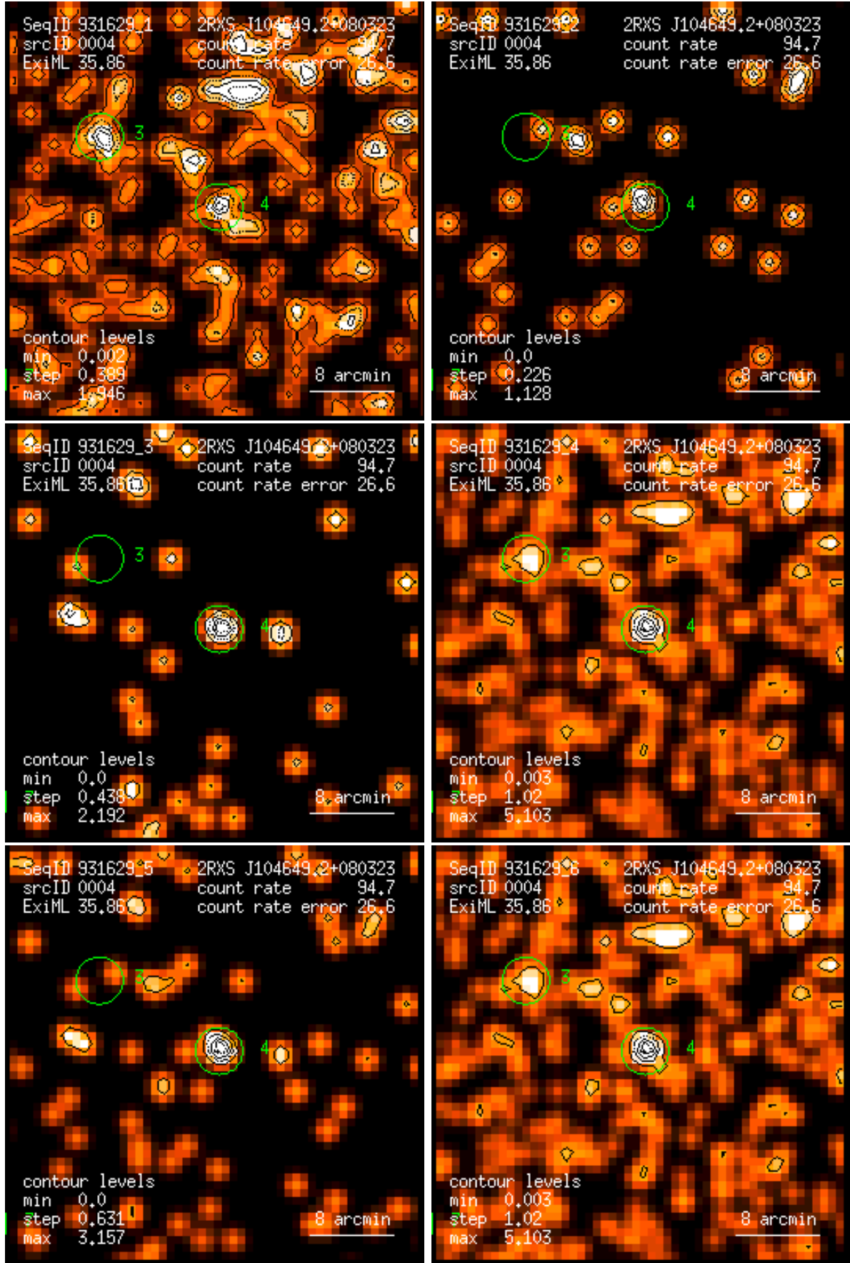
Figure 4: RASS 931629: detection 0004: band rate images, Gaussian filter: (1) PSPC channels 11 – 41, (2) 52 – 90, (3) 91 – 201, (4) 11 – 235, (5) 52 – 201, (6) 11 – 201. Broad band rates in counts/ks. Band rate contour levels in counts/ks/arcmin 2 .
