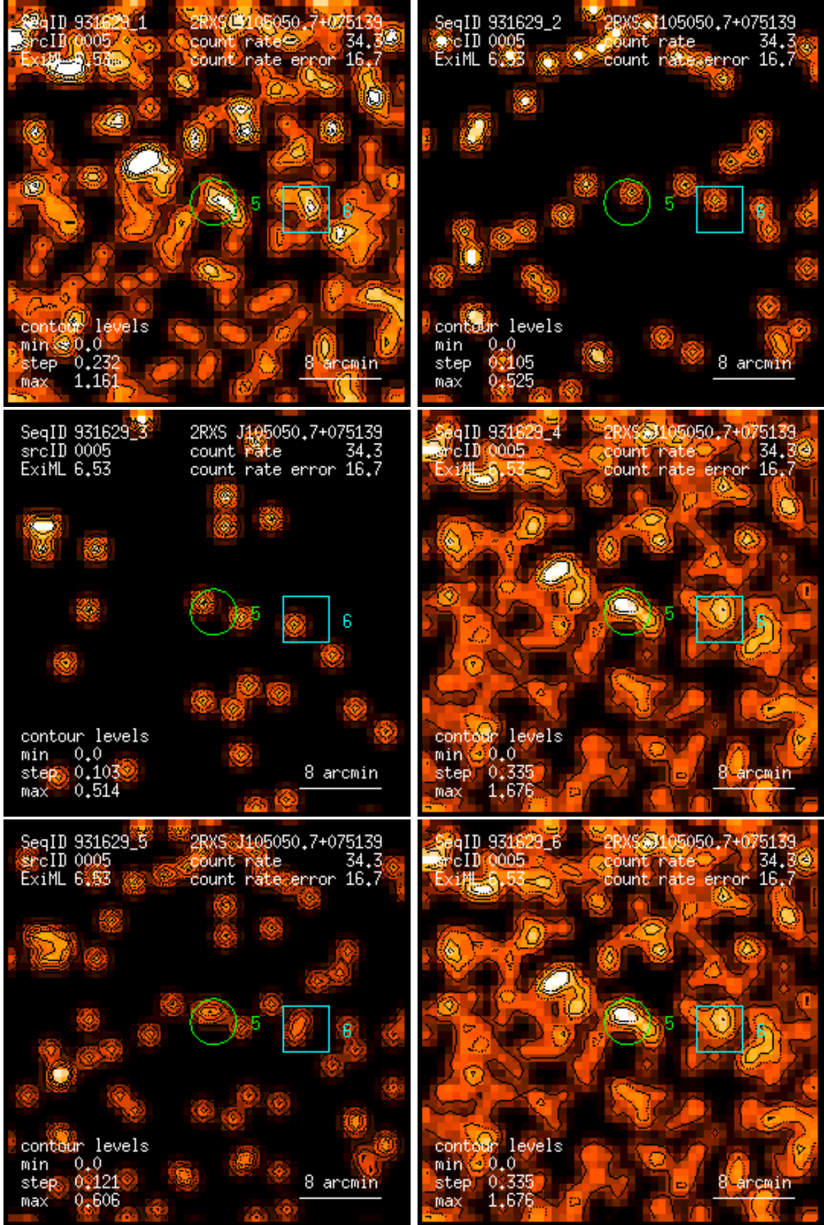
Figure 5: RASS 931629: detection 0005: band rate images, Gaussian filter: (1) PSPC channels 11 – 41, (2) 52 – 90, (3) 91 – 201, (4) 11 – 235, (5) 52 – 201, (6) 11 – 201. Broad band rates in counts/ks. Band rate contour levels in counts/ks/arcmin 2 .
