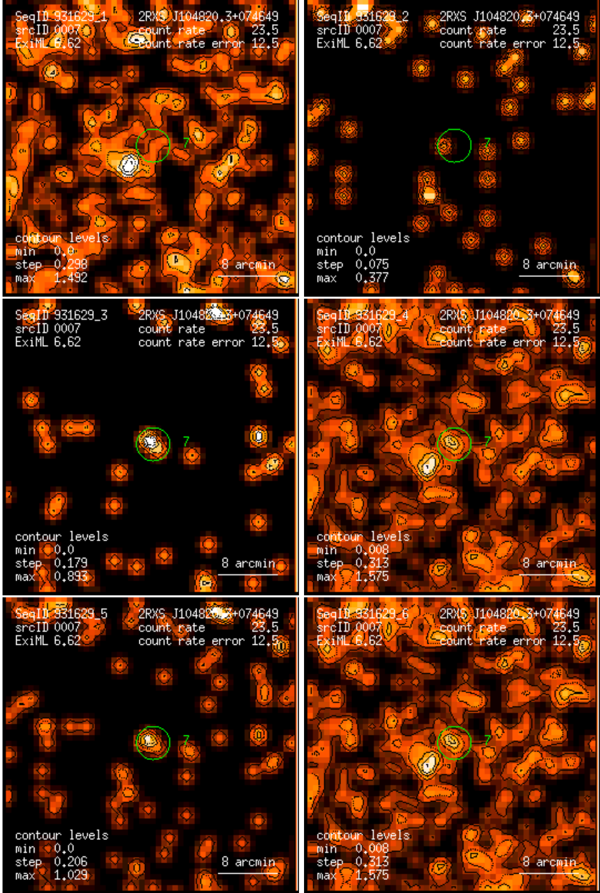
Figure 7: RASS 931629: detection 0007: band rate images, Gaussian filter: (1) PSPC channels 11 – 41, (2) 52 – 90, (3) 91 – 201, (4) 11 – 235, (5) 52 – 201, (6) 11 – 201. Broad band rates in counts/ks. Band rate contour levels in counts/ks/arcmin 2 .
