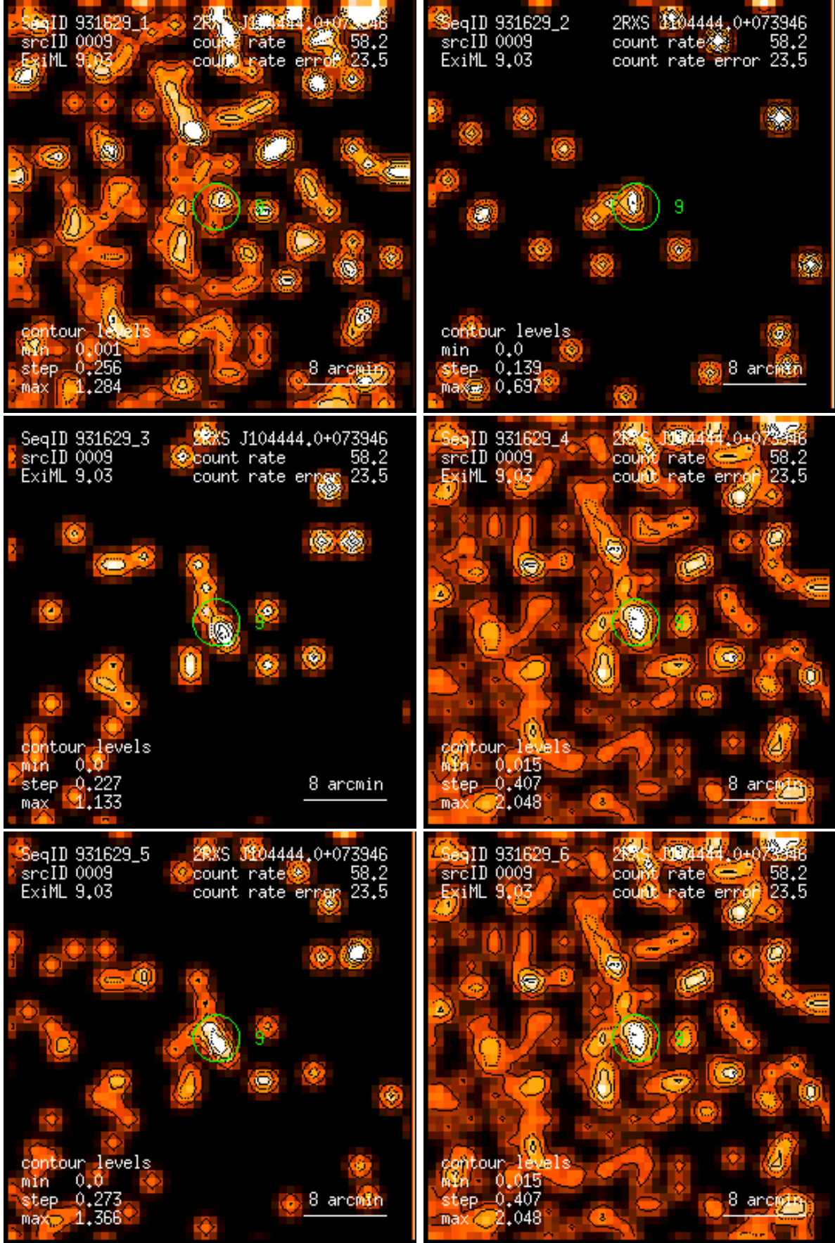
Figure 9: RASS 931629: detection 0009: band rate images, Gaussian filter: (1) PSPC channels 11 – 41, (2) 52 – 90, (3) 91 – 201, (4) 11 – 235, (5) 52 – 201, (6) 11 – 201. Broad band rates in counts/ks. Band rate contour levels in counts/ks/arcmin 2 .
