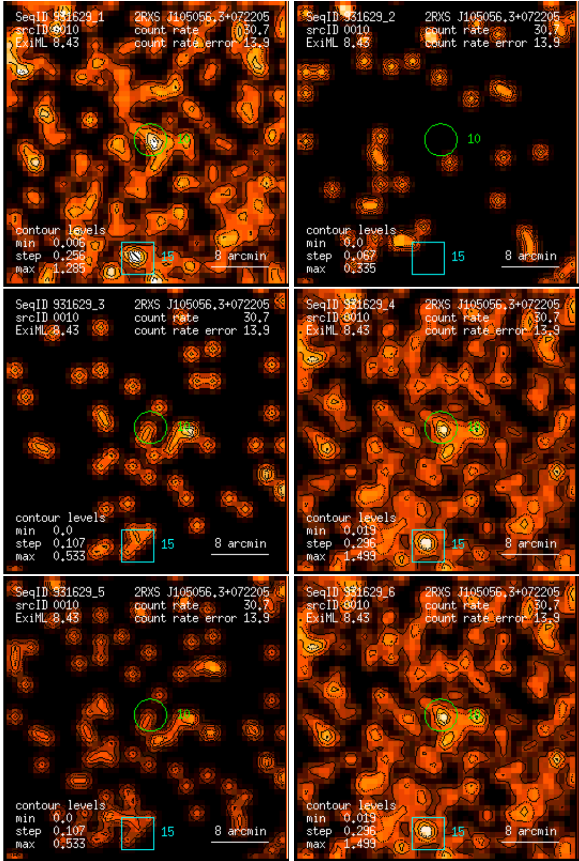
Figure 10: RASS 931629: detection 0010: band rate images, Gaussian filter: (1) PSPC channels 11 – 41, (2) 52 – 90, (3) 91 – 201, (4) 11 – 235, (5) 52 – 201, (6) 11 – 201. Broad band rates in counts/ks. Band rate contour levels in counts/ks/arcmin 2 .
