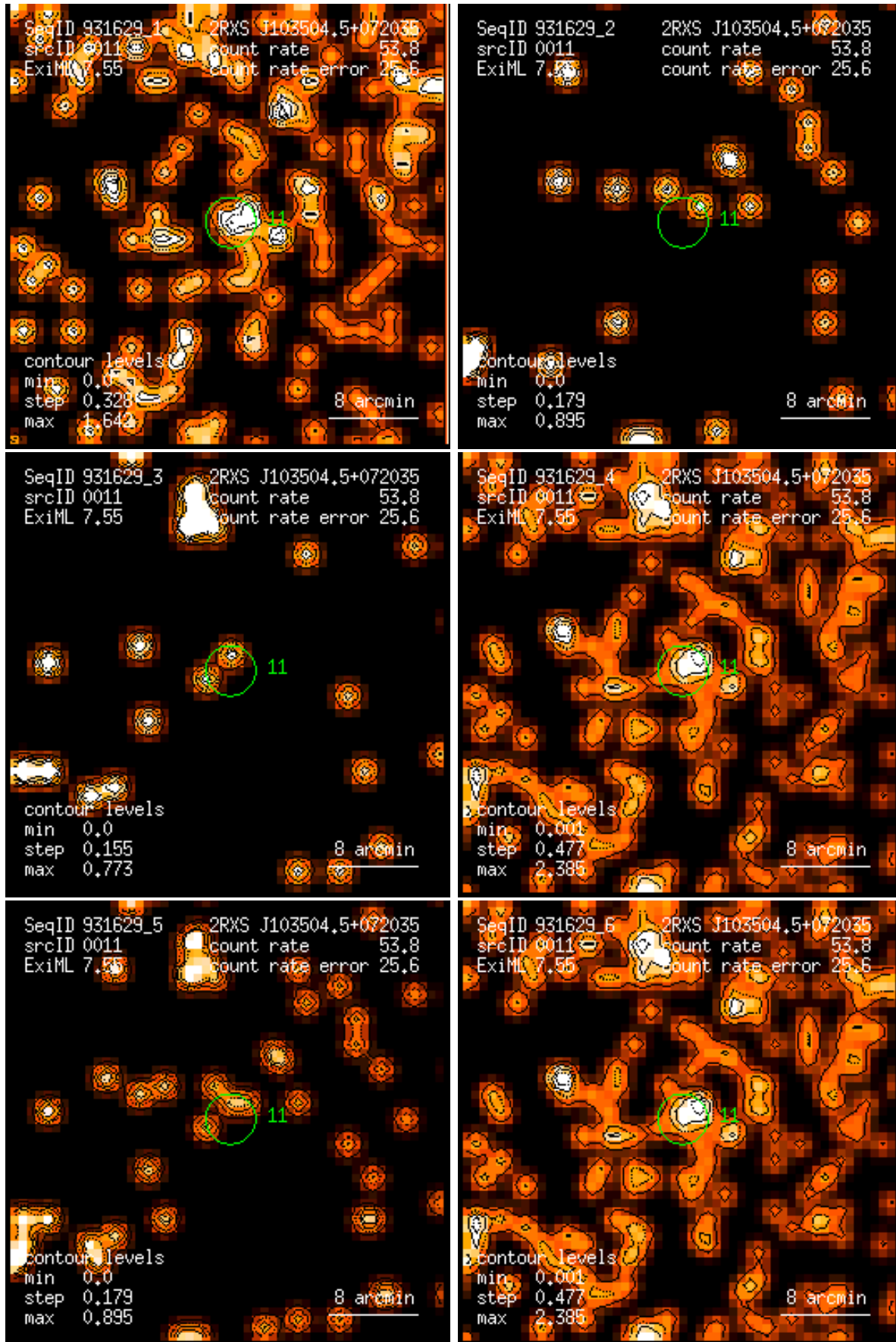
Figure 11: RASS 931629: detection 0011: band rate images, Gaussian filter: (1) PSPC channels 11 – 41, (2) 52 – 90, (3) 91 – 201, (4) 11 – 235, (5) 52 – 201, (6) 11 – 201. Broad band rates in counts/ks. Band rate contour levels in counts/ks/arcmin 2 .
