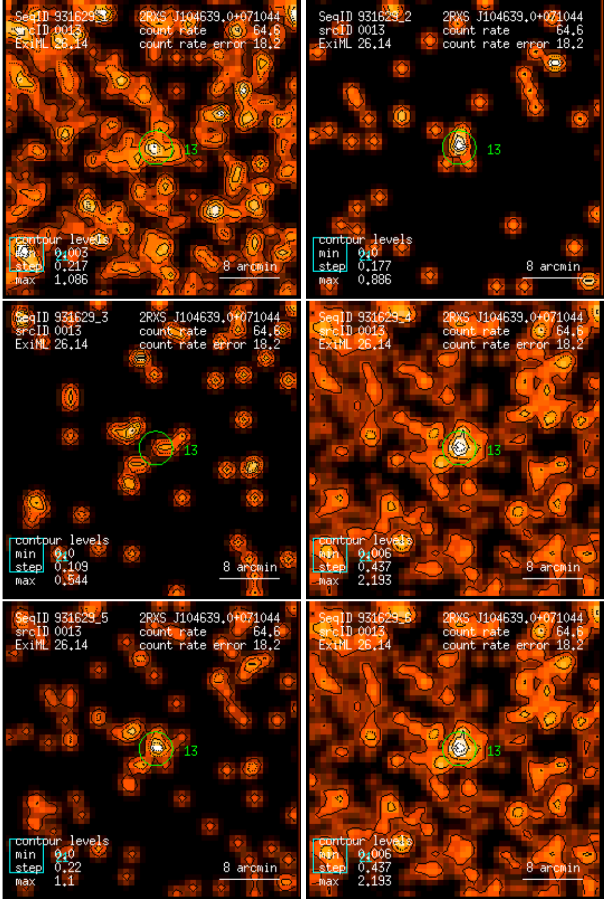
Figure 13: RASS 931629: detection 0013: band rate images, Gaussian filter: (1) PSPC channels 11 – 41, (2) 52 – 90, (3) 91 – 201, (4) 11 – 235, (5) 52 – 201, (6) 11 – 201. Broad band rates in counts/ks. Band rate contour levels in counts/ks/arcmin 2 .
