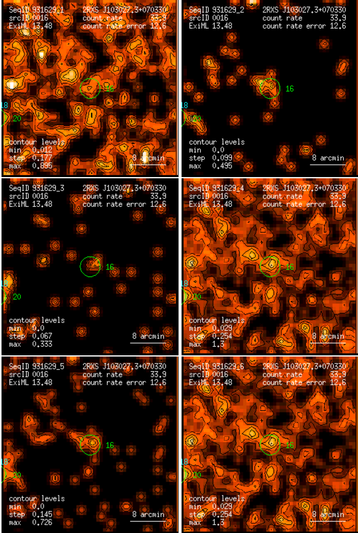
Figure 16: RASS 931629: detection 0016: band rate images, Gaussian filter: (1) PSPC channels 11 – 41, (2) 52 – 90, (3) 91 – 201, (4) 11 – 235, (5) 52 – 201, (6) 11 – 201. Broad band rates in counts/ks. Band rate contour levels in counts/ks/arcmin 2 .
