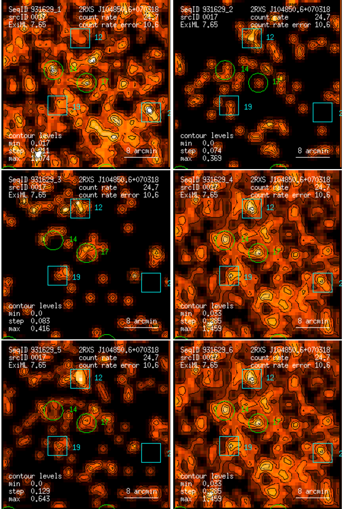
Figure 17: RASS 931629: detection 0017: band rate images, Gaussian filter: (1) PSPC channels 11 – 41, (2) 52 – 90, (3) 91 – 201, (4) 11 – 235, (5) 52 – 201, (6) 11 – 201. Broad band rates in counts/ks. Band rate contour levels in counts/ks/arcmin 2 .
