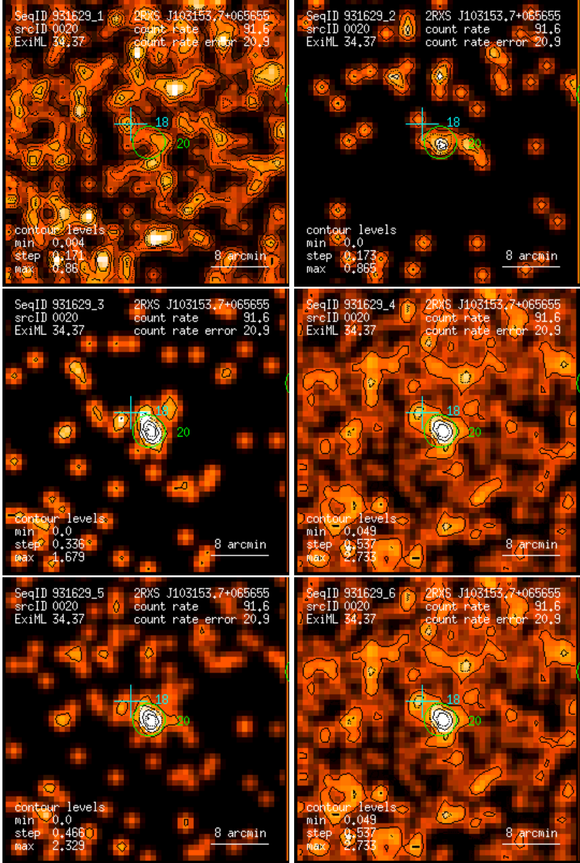
Figure 20: RASS 931629: detection 0020: band rate images, Gaussian filter: (1) PSPC channels 11 – 41, (2) 52 – 90, (3) 91 – 201, (4) 11 – 235, (5) 52 – 201, (6) 11 – 201. Broad band rates in counts/ks. Band rate contour levels in counts/ks/arcmin 2 .
