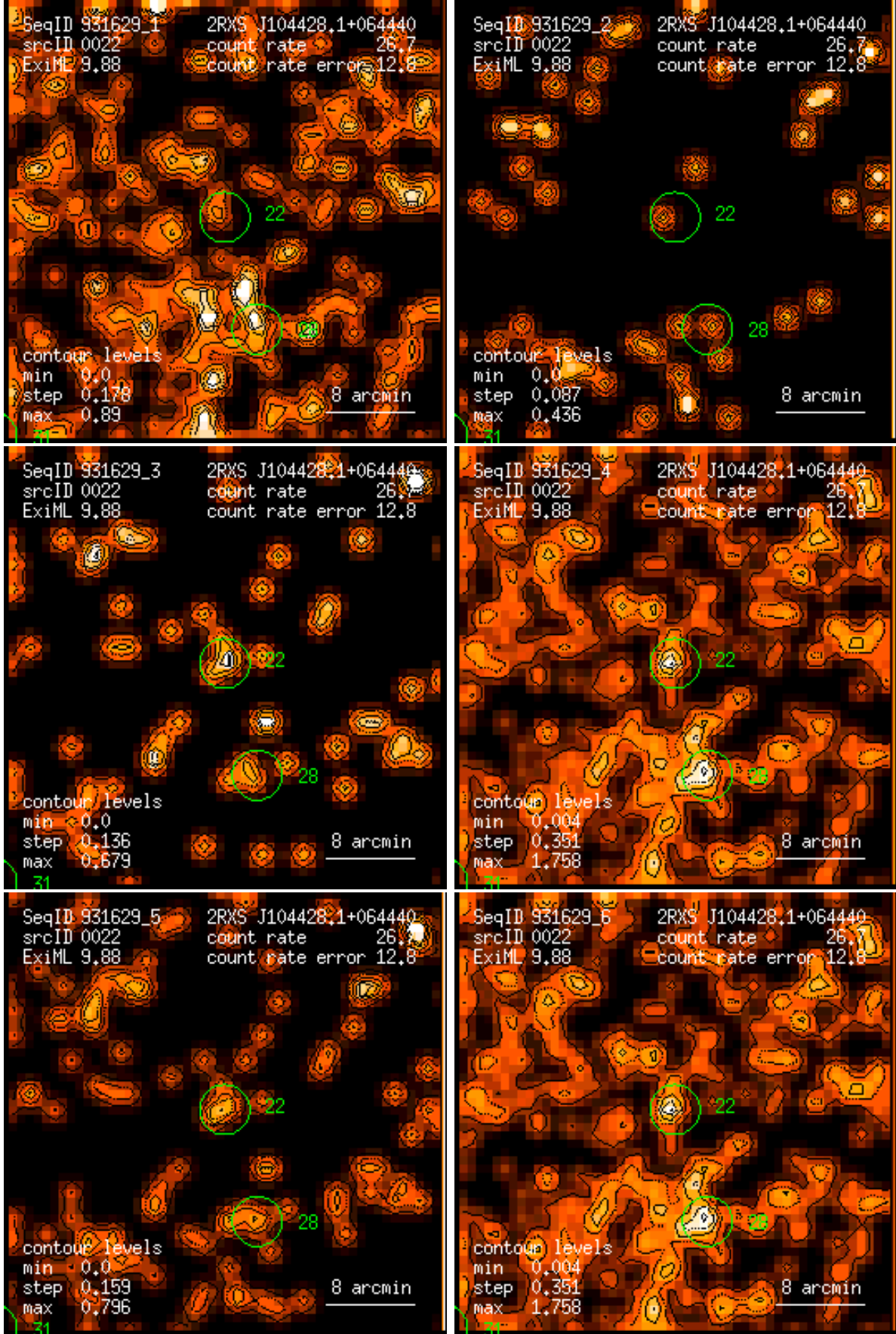
Figure 22: RASS 931629: detection 0022: band rate images, Gaussian filter: (1) PSPC channels 11 – 41, (2) 52 – 90, (3) 91 – 201, (4) 11 – 235, (5) 52 – 201, (6) 11 – 201. Broad band rates in counts/ks. Band rate contour levels in counts/ks/arcmin 2 .
