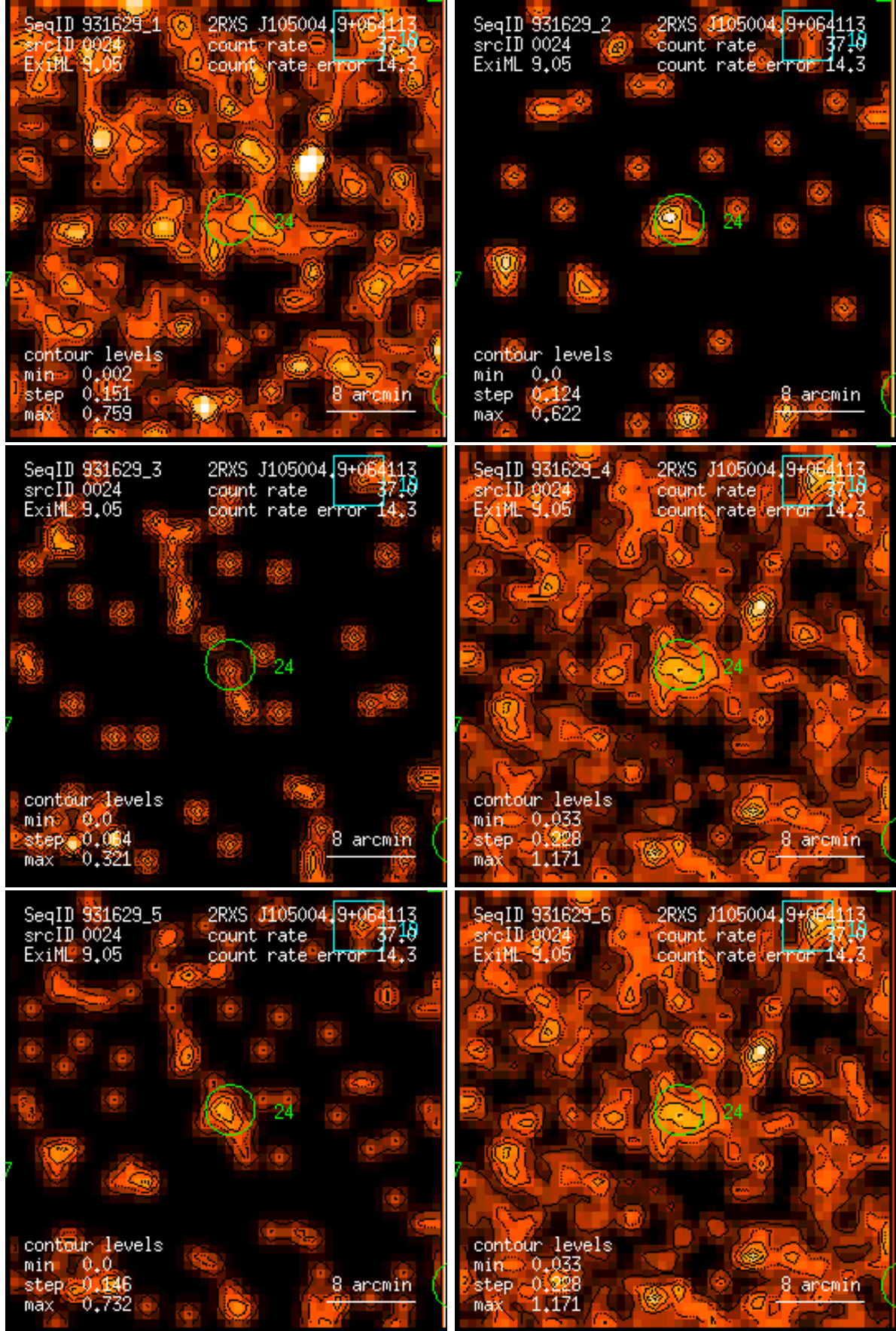
Figure 24: RASS 931629: detection 0024: band rate images, Gaussian filter: (1) PSPC channels 11 – 41, (2) 52 – 90, (3) 91 – 201, (4) 11 – 235, (5) 52 – 201, (6) 11 – 201. Broad band rates in counts/ks. Band rate contour levels in counts/ks/arcmin 2 .
