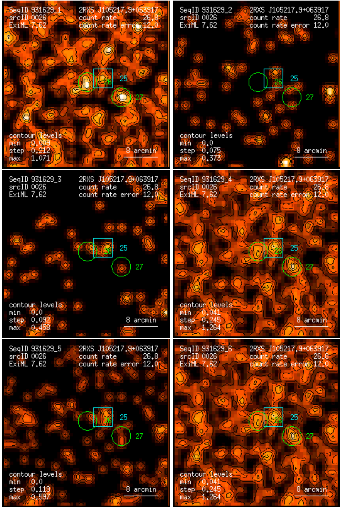
Figure 26: RASS 931629: detection 0026: band rate images, Gaussian filter: (1) PSPC channels 11 – 41, (2) 52 – 90, (3) 91 – 201, (4) 11 – 235, (5) 52 – 201, (6) 11 – 201. Broad band rates in counts/ks. Band rate contour levels in counts/ks/arcmin 2 .
