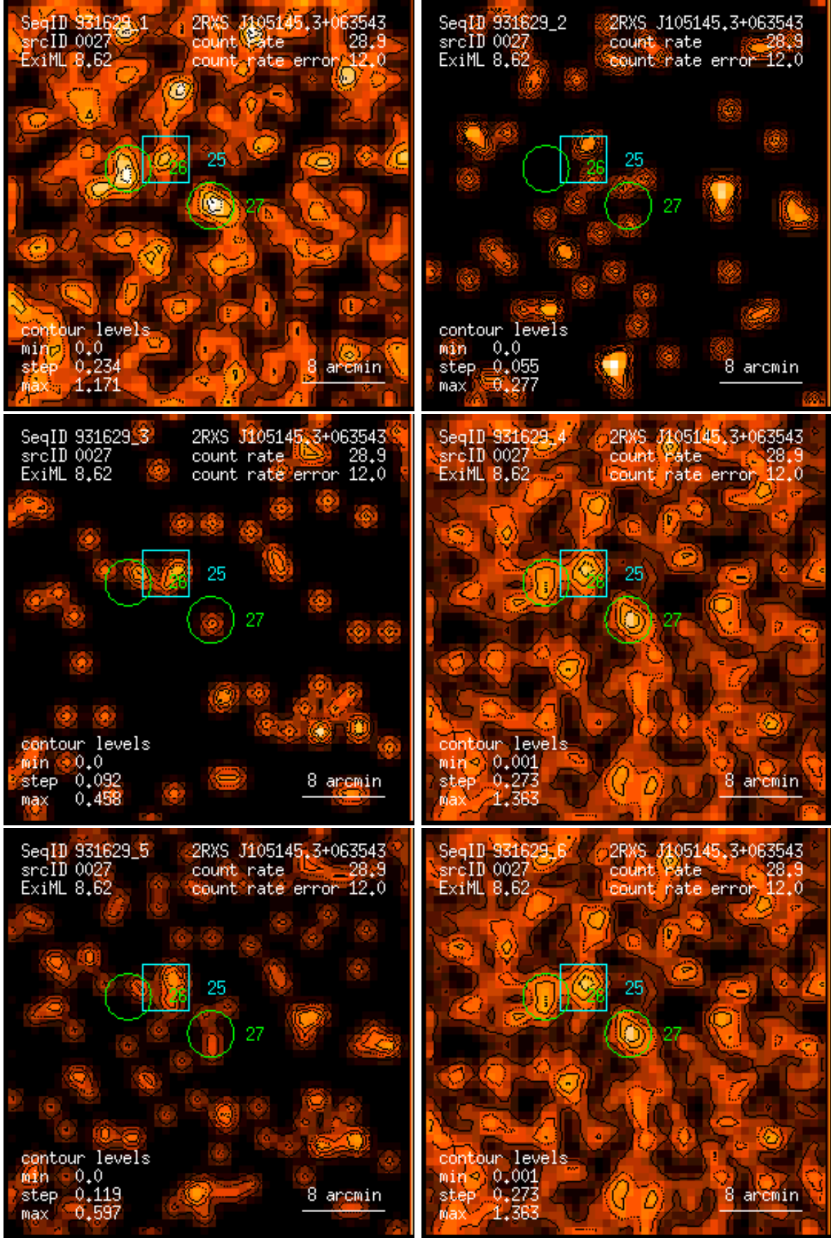
Figure 27: RASS 931629: detection 0027: band rate images, Gaussian filter: (1) PSPC channels 11 – 41, (2) 52 – 90, (3) 91 – 201, (4) 11 – 235, (5) 52 – 201, (6) 11 – 201. Broad band rates in counts/ks. Band rate contour levels in counts/ks/arcmin 2 .
