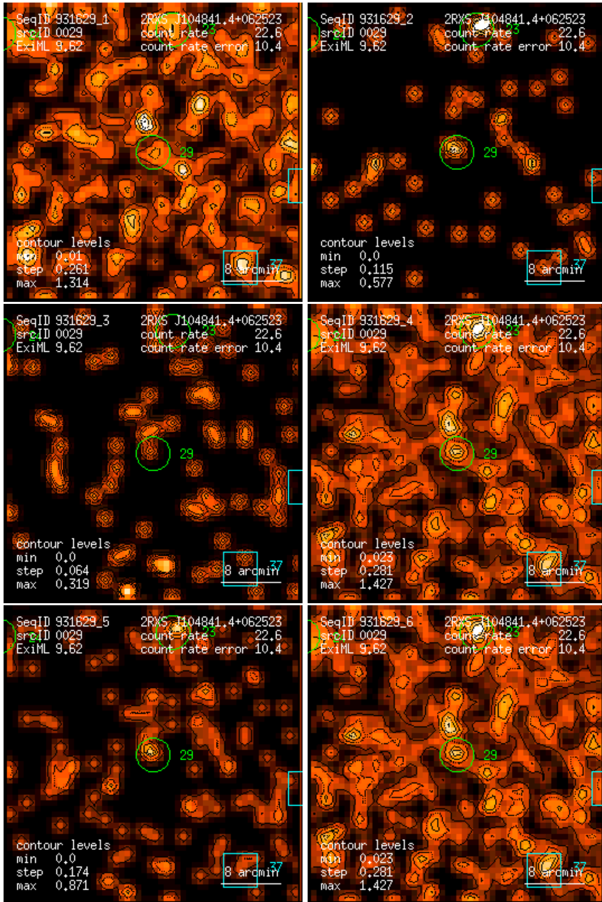
Figure 29: RASS 931629: detection 0029: band rate images, Gaussian filter: (1) PSPC channels 11 – 41, (2) 52 – 90, (3) 91 – 201, (4) 11 – 235, (5) 52 – 201, (6) 11 – 201. Broad band rates in counts/ks. Band rate contour levels in counts/ks/arcmin 2 .
