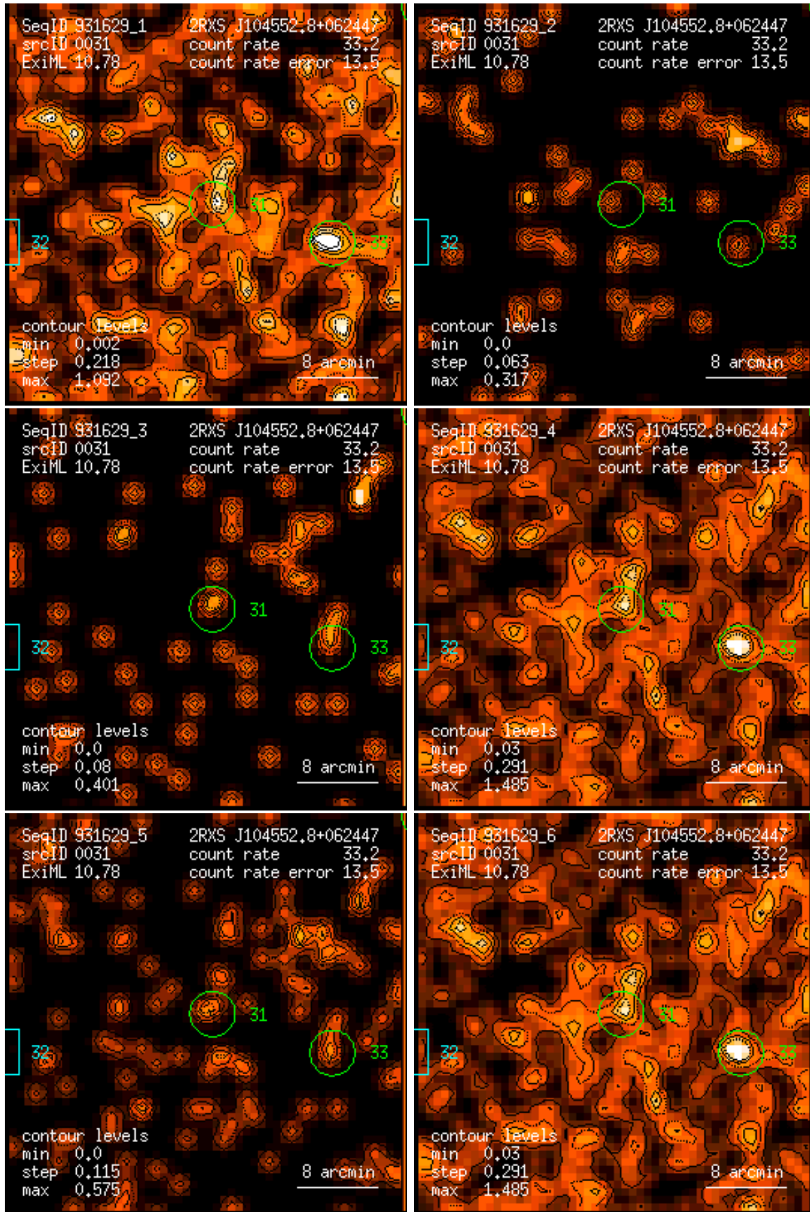
Figure 31: RASS 931629: detection 0031: band rate images, Gaussian filter: (1) PSPC channels 11 – 41, (2) 52 – 90, (3) 91 – 201, (4) 11 – 235, (5) 52 – 201, (6) 11 – 201. Broad band rates in counts/ks. Band rate contour levels in counts/ks/arcmin 2 .
